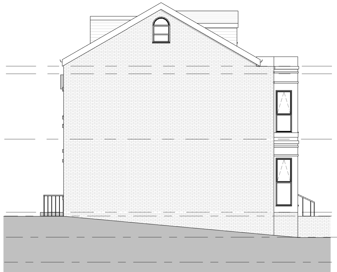
2 Existing South Elevation 1 : 100
