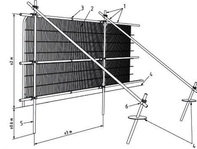
BS5837 (2012) Tree Protective Fencing Standard Detail.
