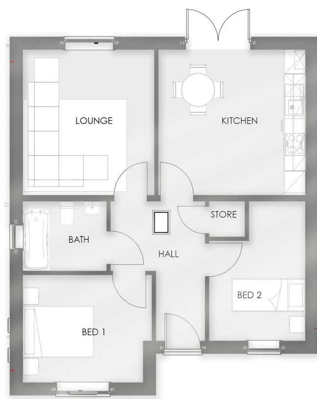
GROUND FLOOR 1 : 100
