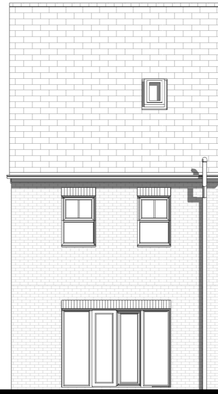
REAR ELEVATION 1 : 100
