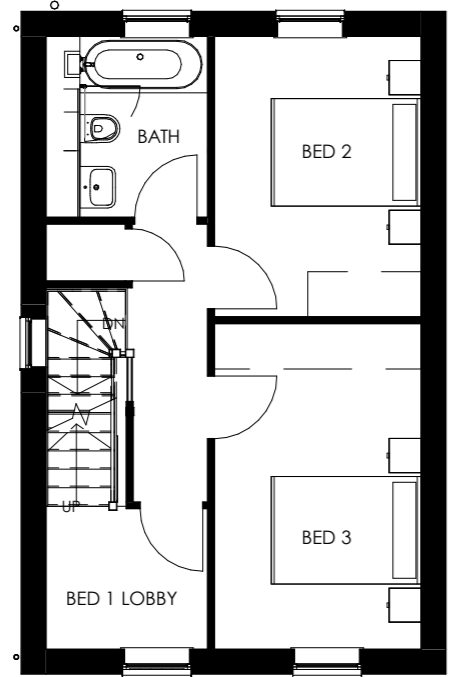
FIRST FLOOR LAYOUT 1 : 100
