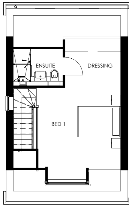
SECOND FLOOR LAYOUT 1 : 100
