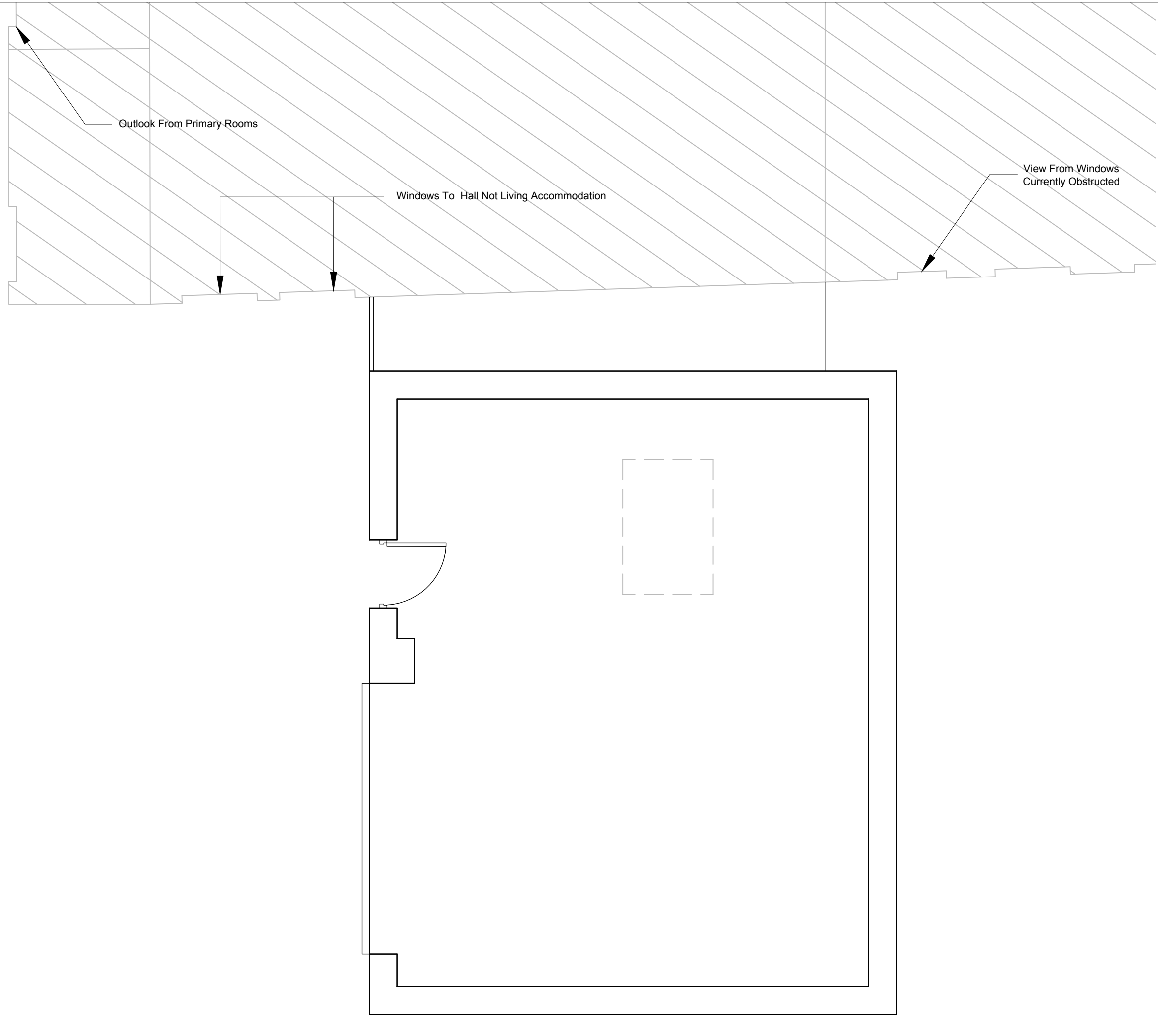
Existing Floor Plan 1:50
