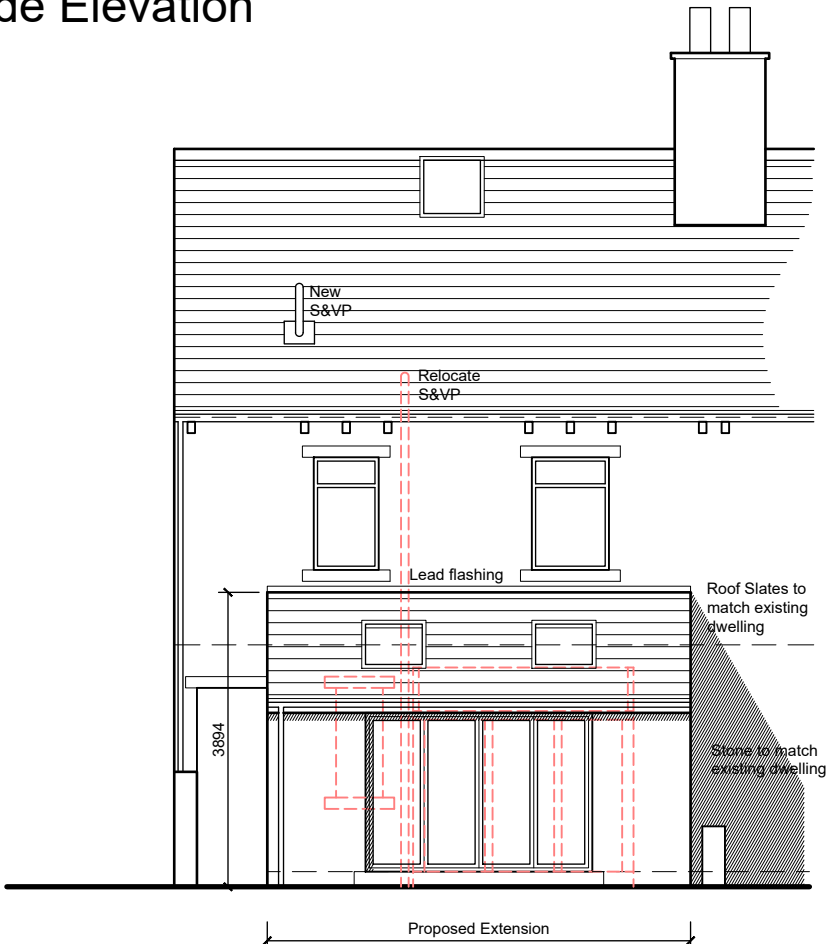
Rear Elevation
