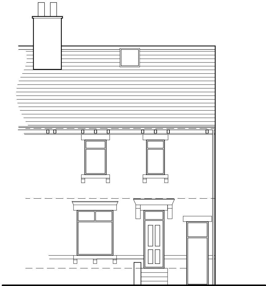
Front Elevation
