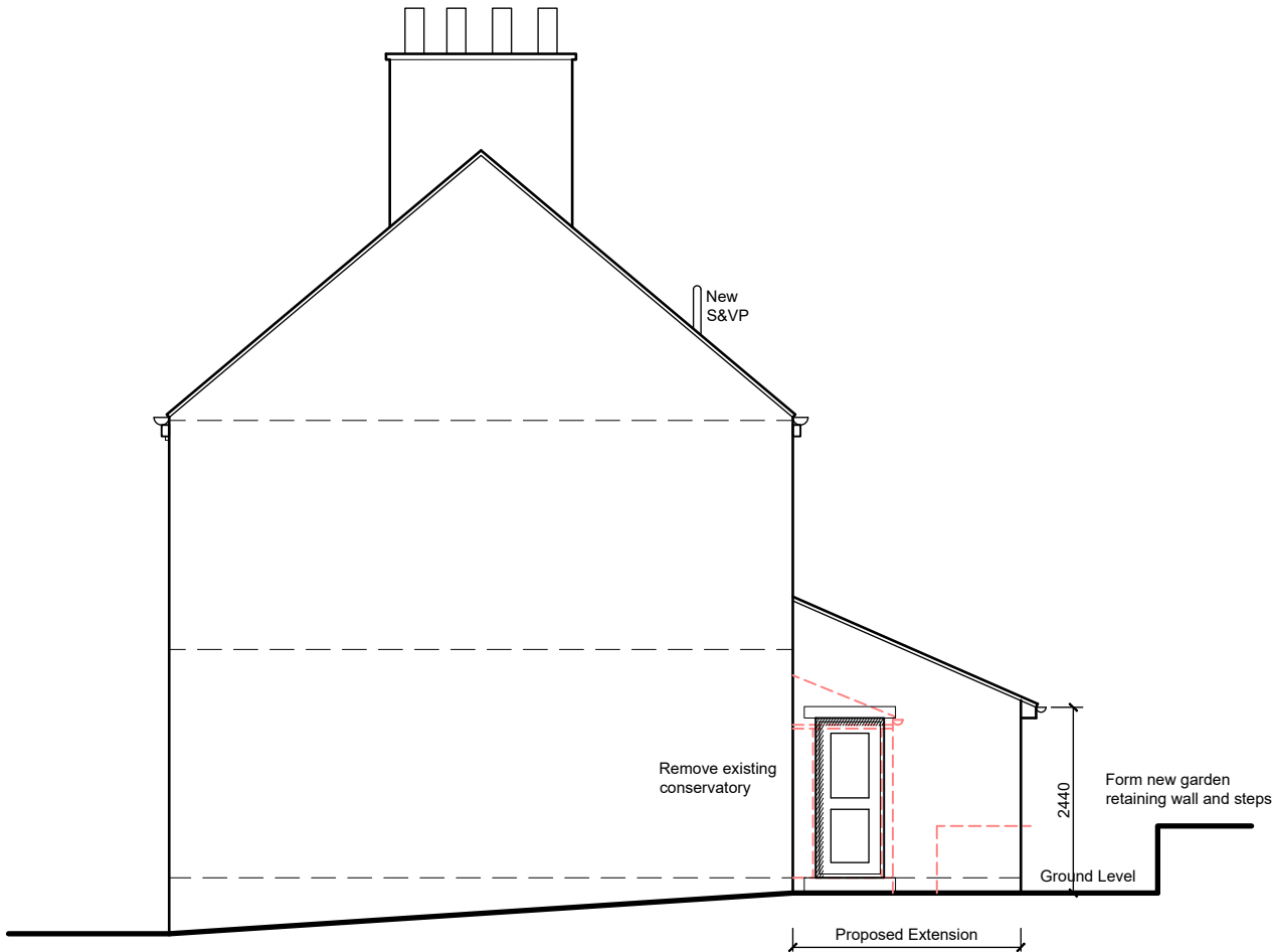
Side Elevation
