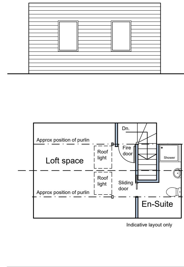
Roof Space Plan
