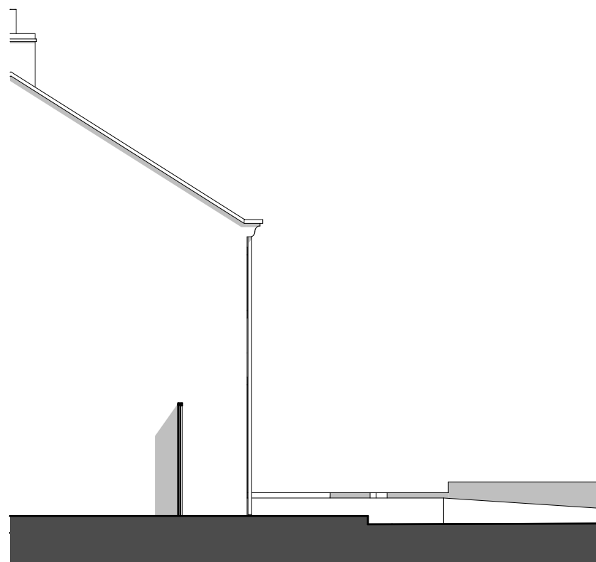
South West Elevation 1:100
