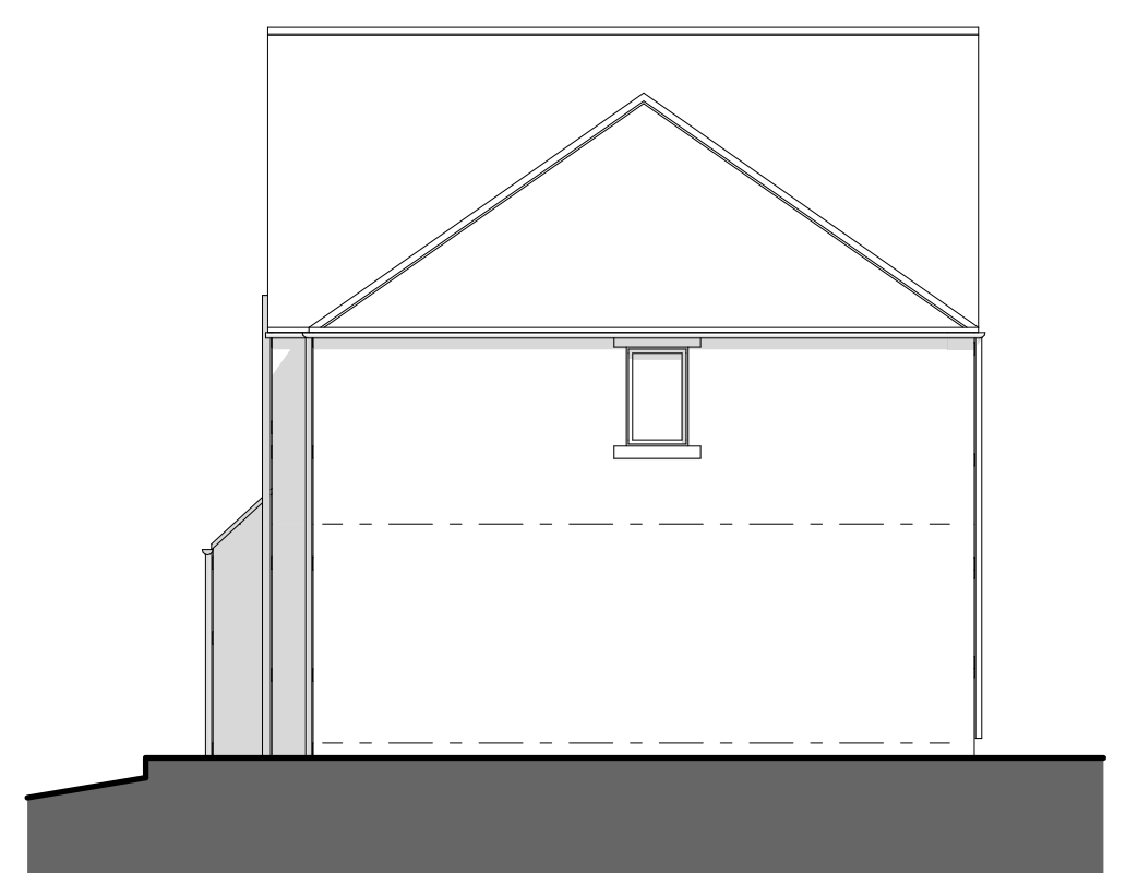
West Elevation 1:100
