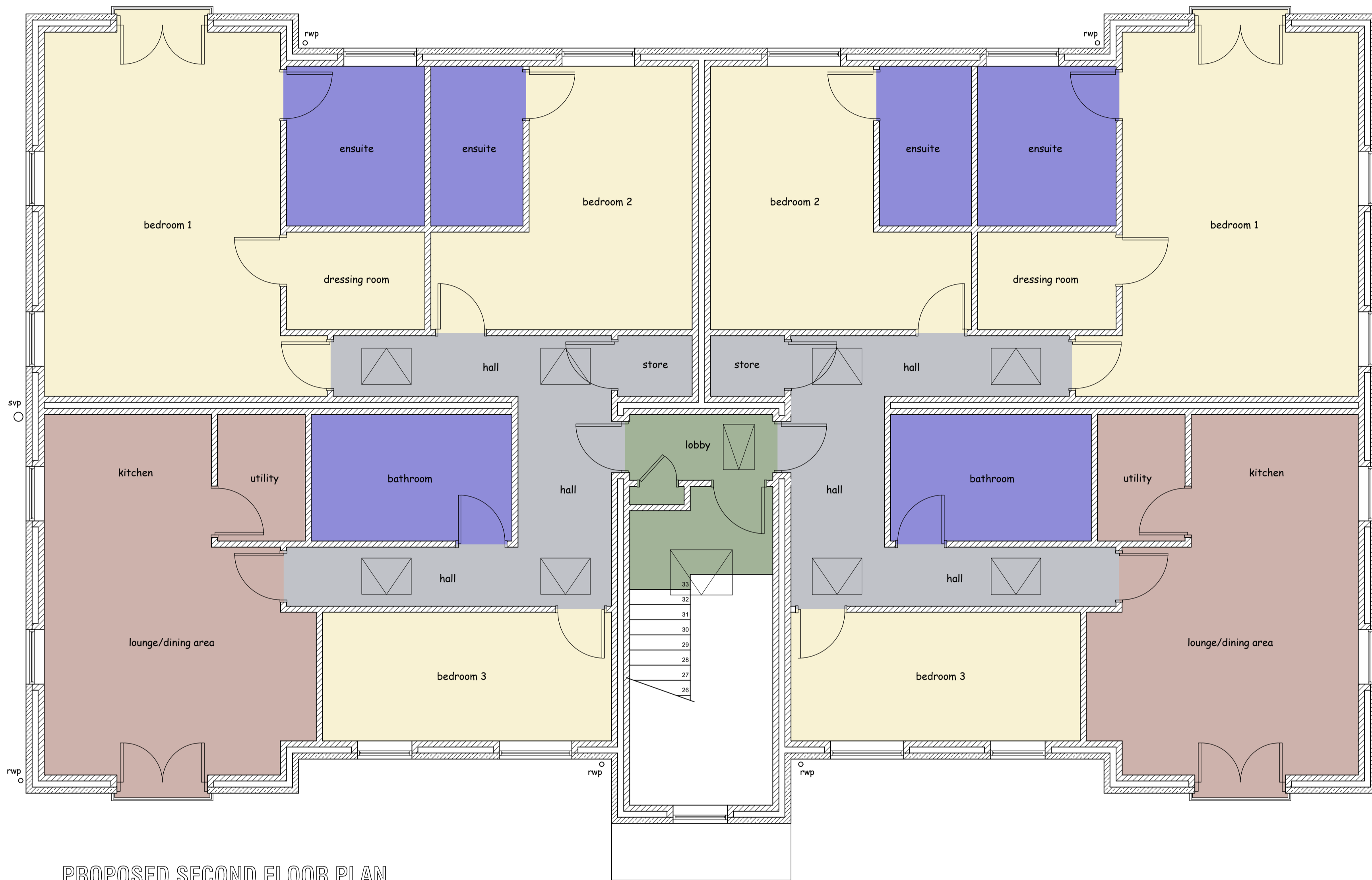
PROPOSED SECOND FLOOR PLAN (1/50 SCALE)
