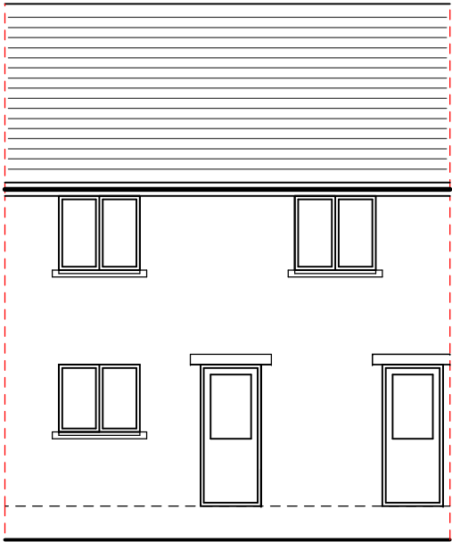
rear (north west) elevation
