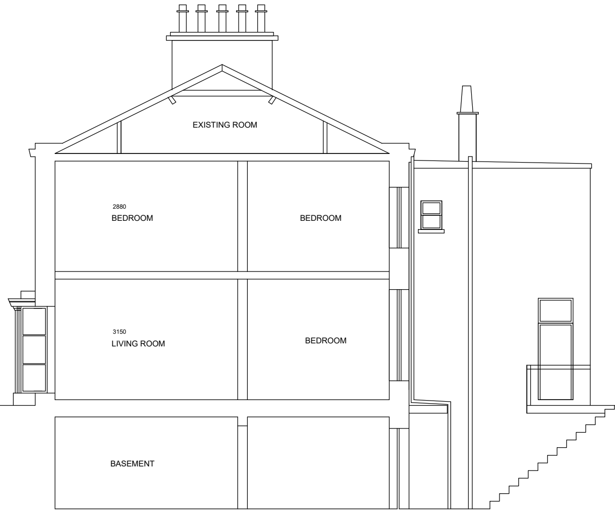
SECTION B-B
