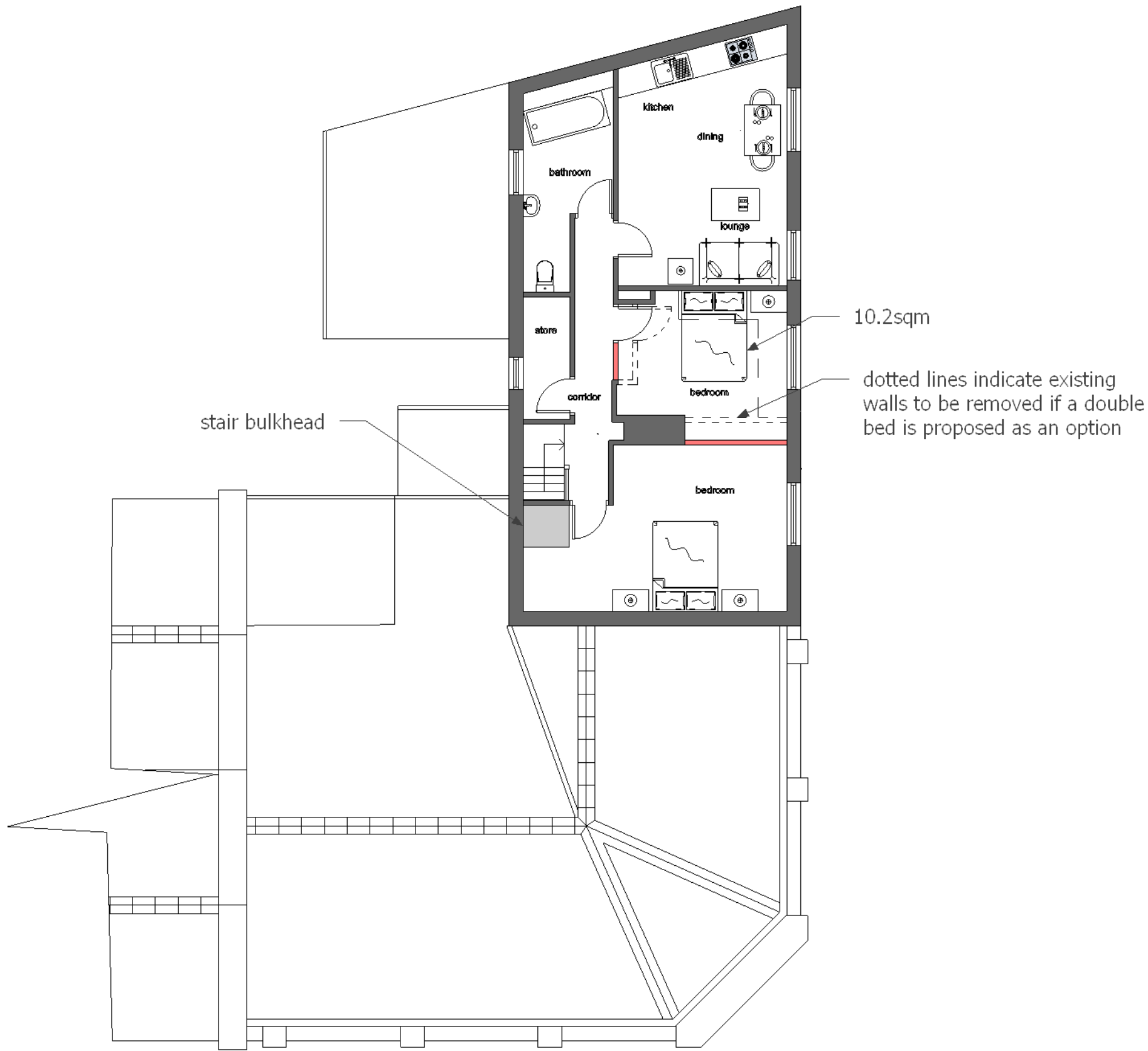
proposed first floor (option 2 if doubled bed)
