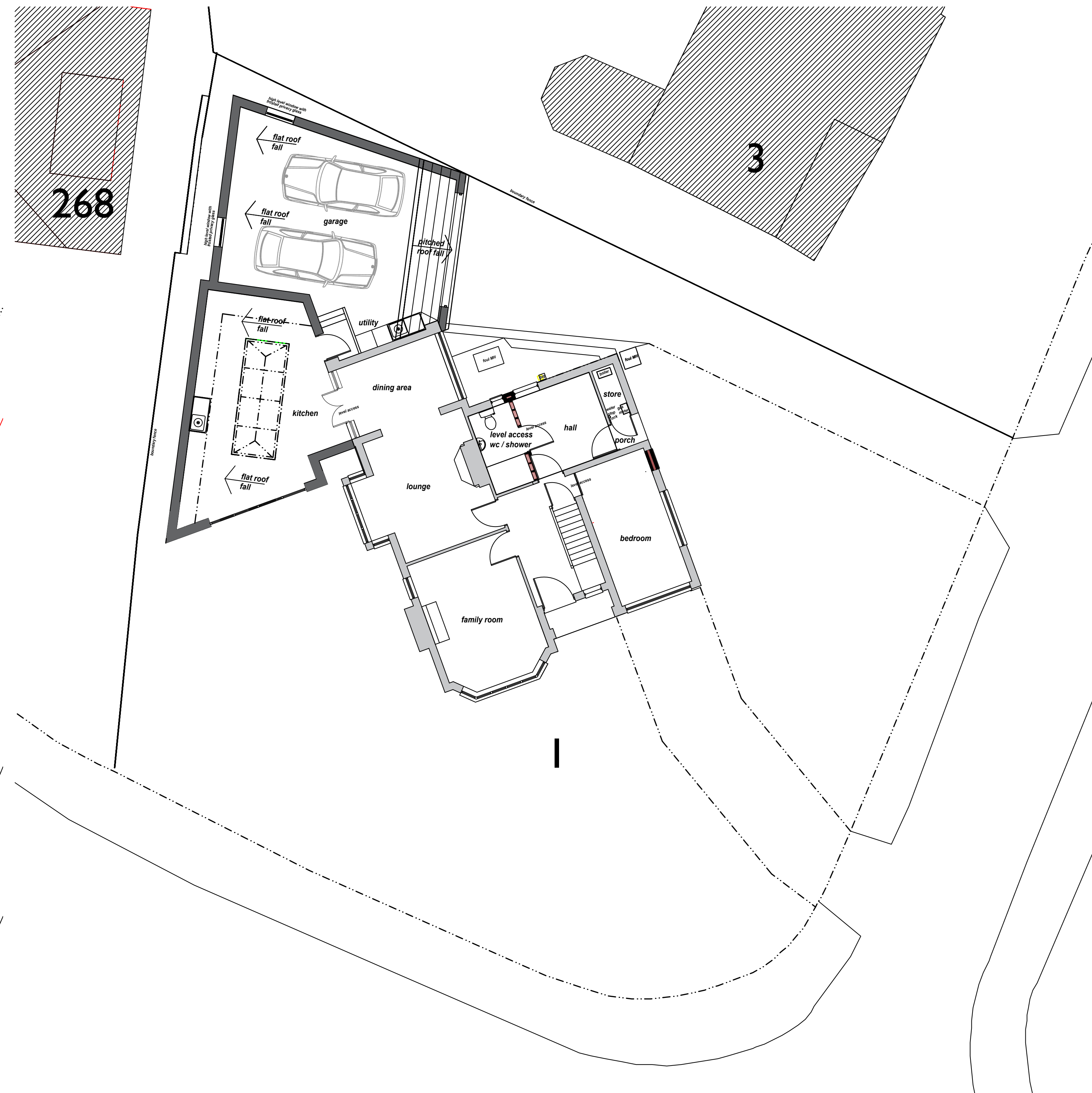
Proposed Ground Floor & Site Plan
