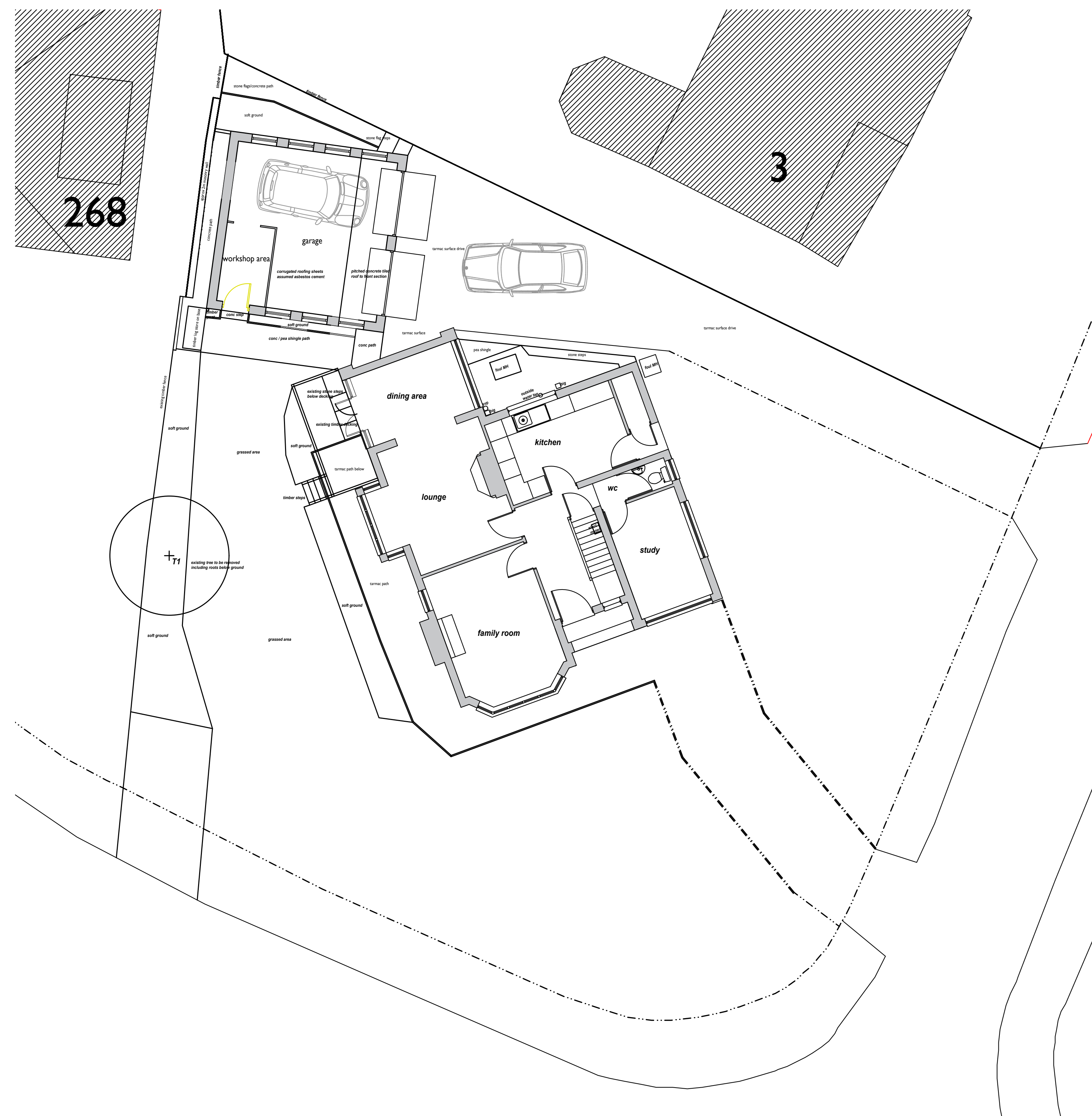
Existing Ground Floor & Site Plan
