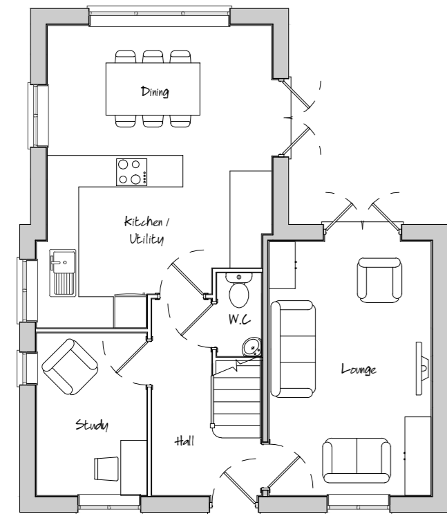
GROUND FLOOR LAYOUT
