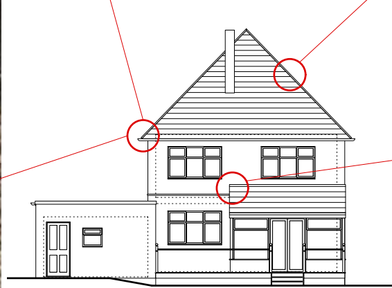
Rear Elevation As Existing
