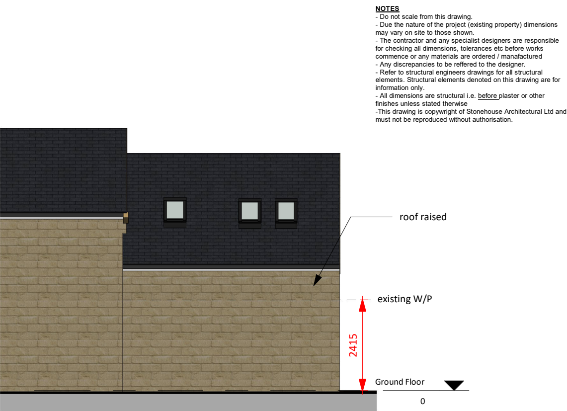
11 Rear Proposed 1 : 100
