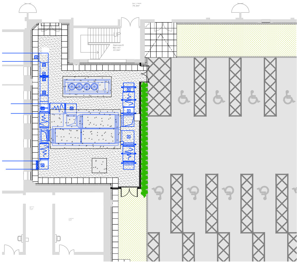
Key Plan as Proposed Scale 1:200
