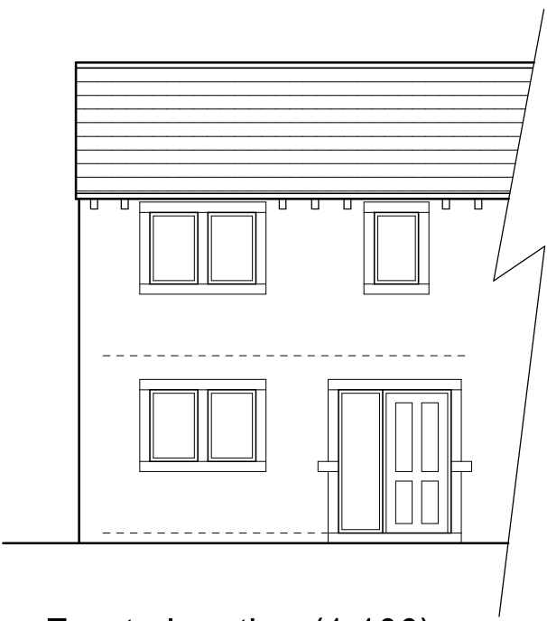
Front elevation (1:100)
