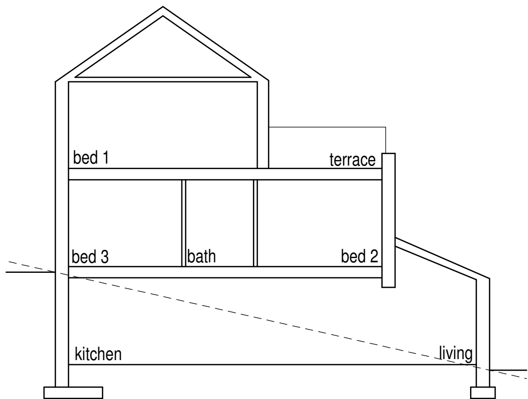
Section 1 House Type C1 (1:100)
