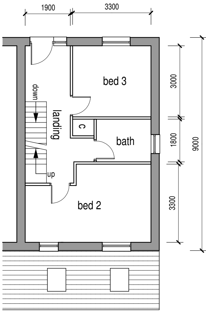
First Floor (1:100)
