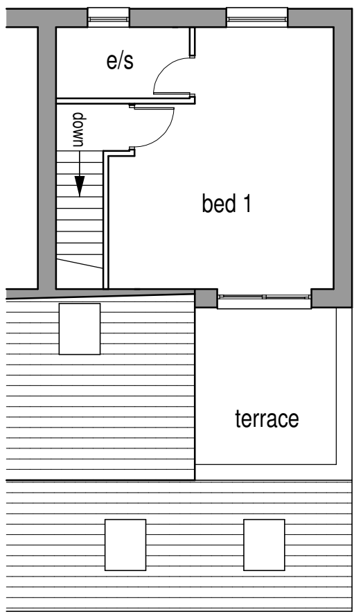
Second Floor (1:100)
