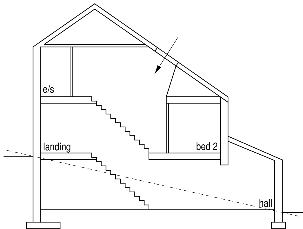
Section 2 House Type C1 (1:100)
