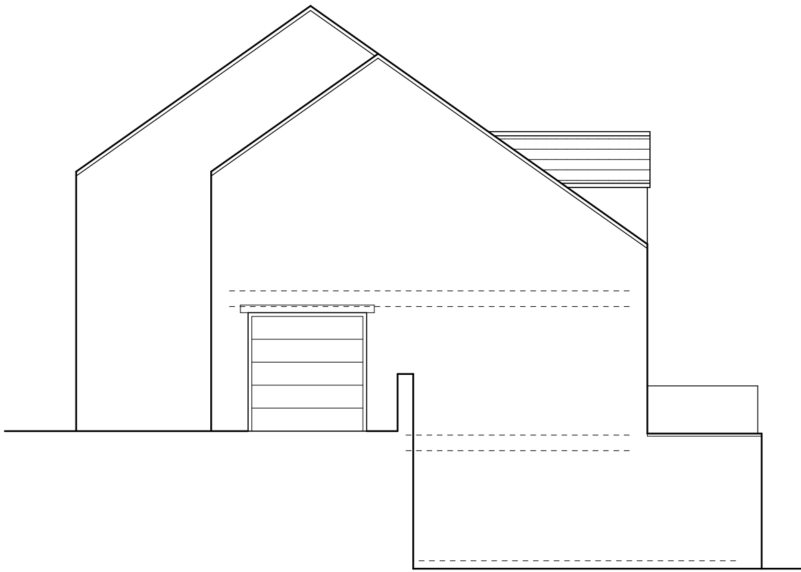
Side elevation (1:100)
