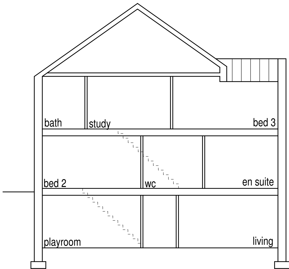
Section 1 (1:100)
