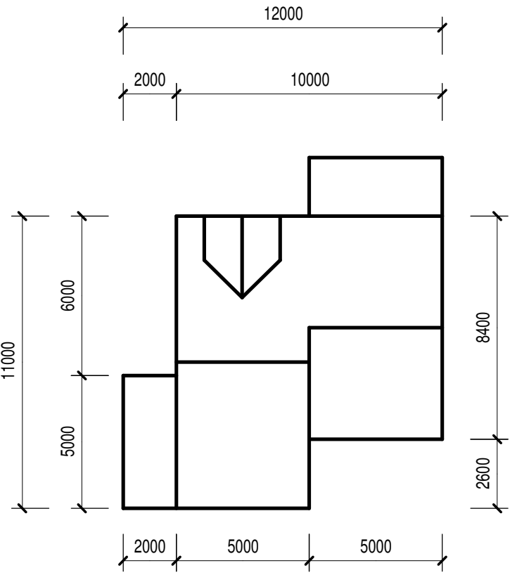
A1 roof plan (1:200)
