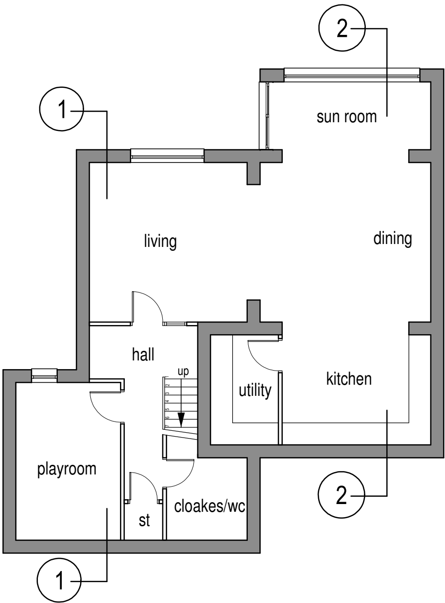
Ground Floor (1:100)
