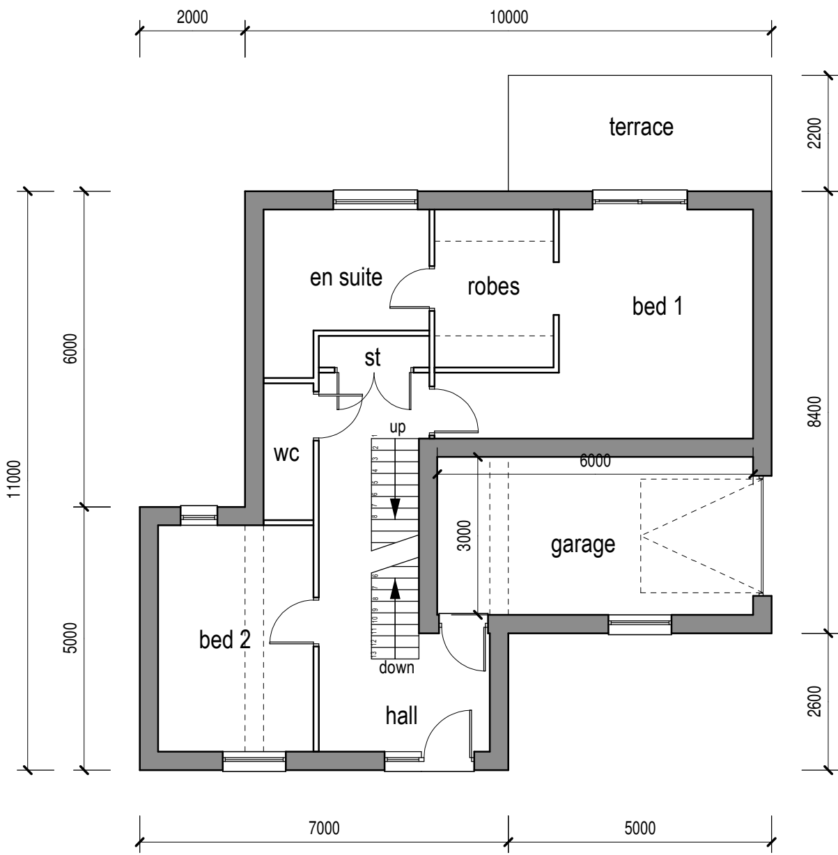
First Floor (1:100)
