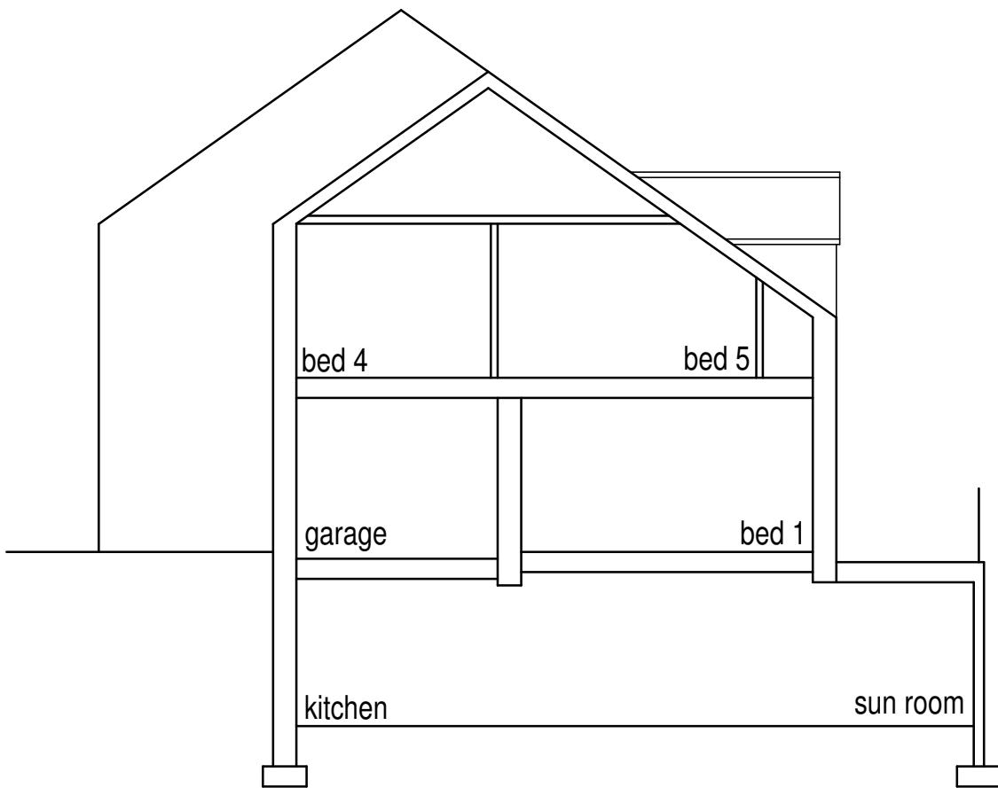
Section 2 (1:100)
