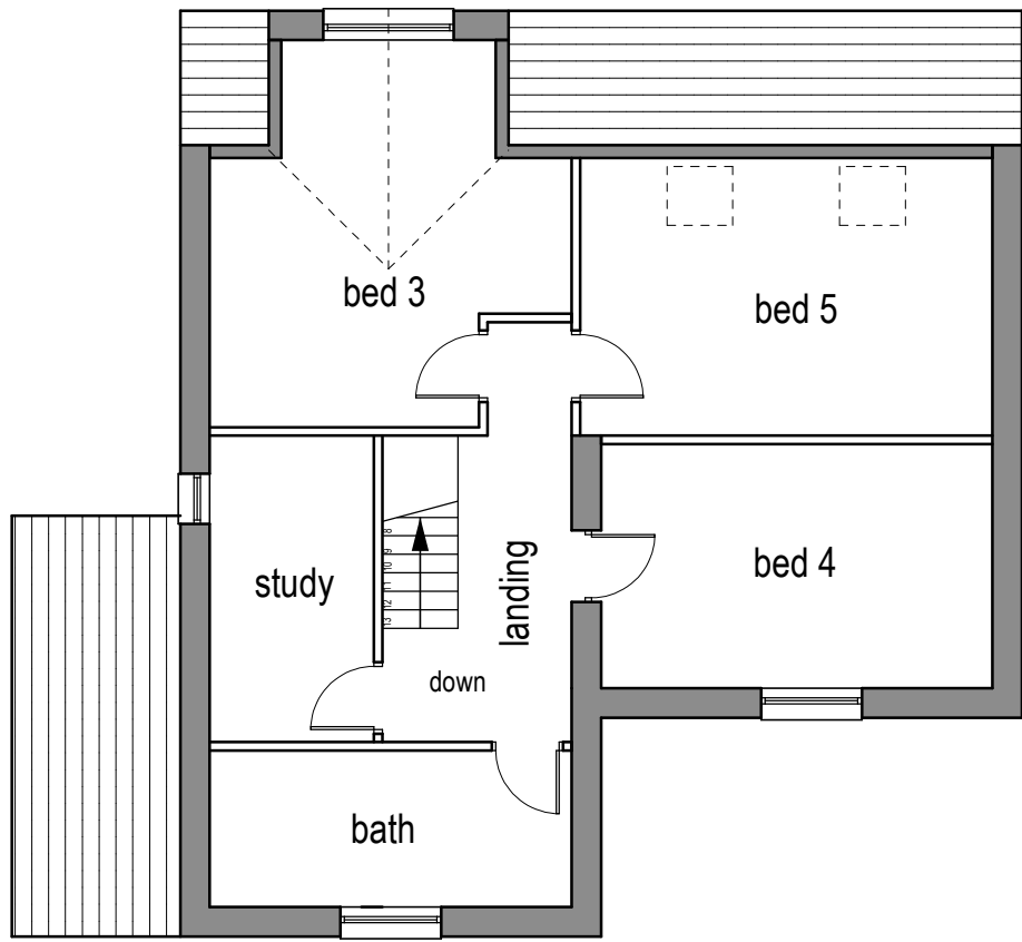
Second Floor (1:100)
