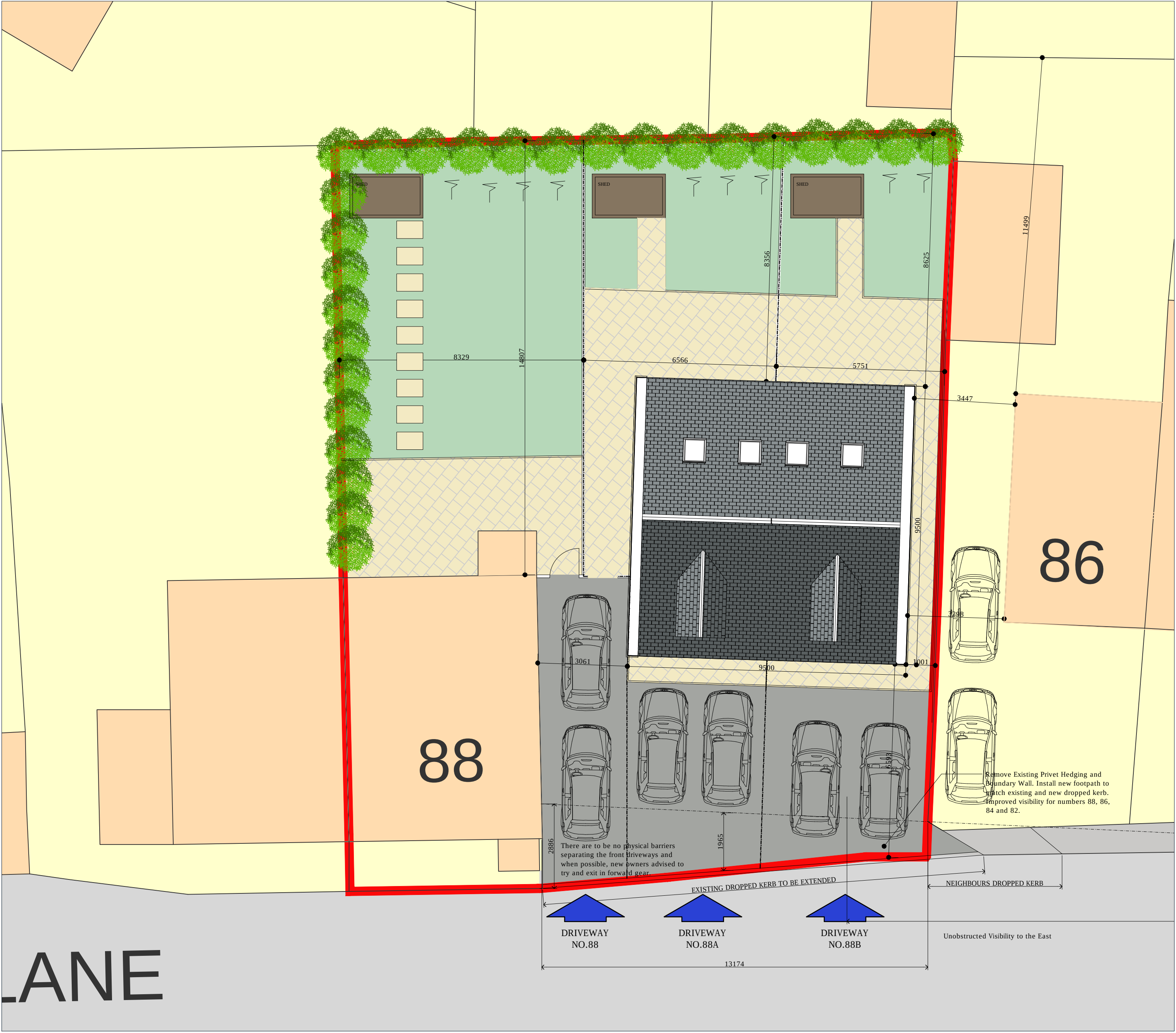
3 Proposed Site Layout
