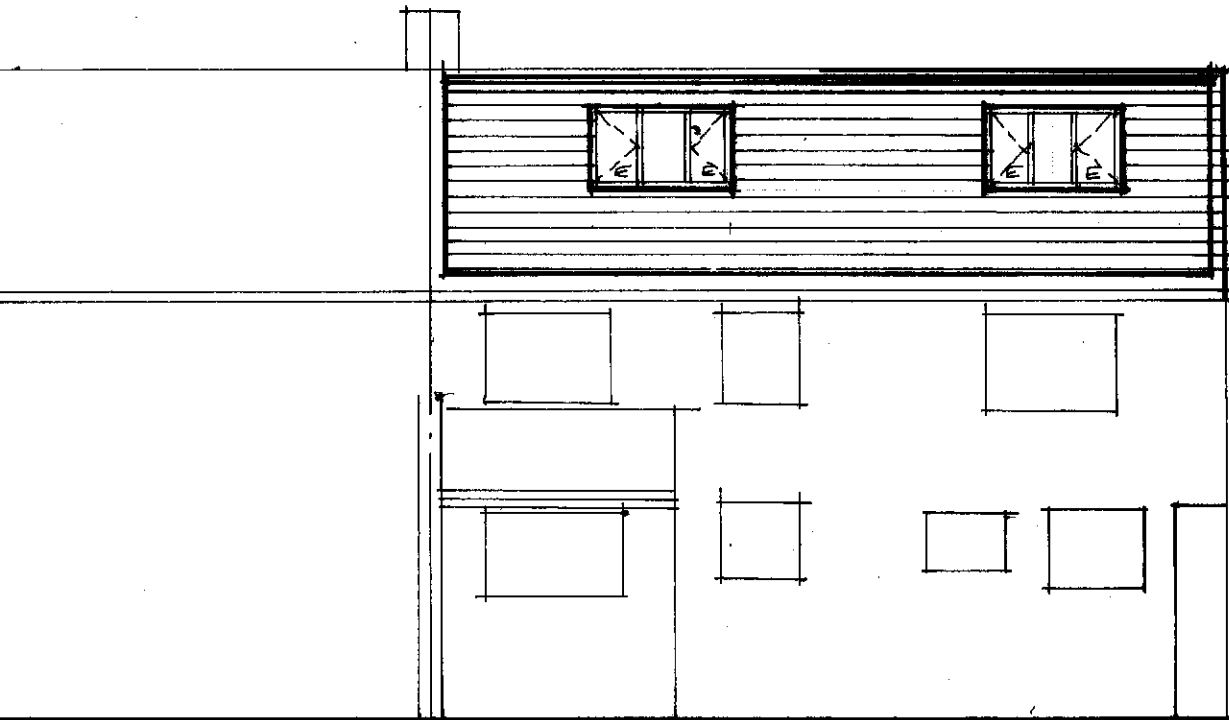
REAR 1:100
