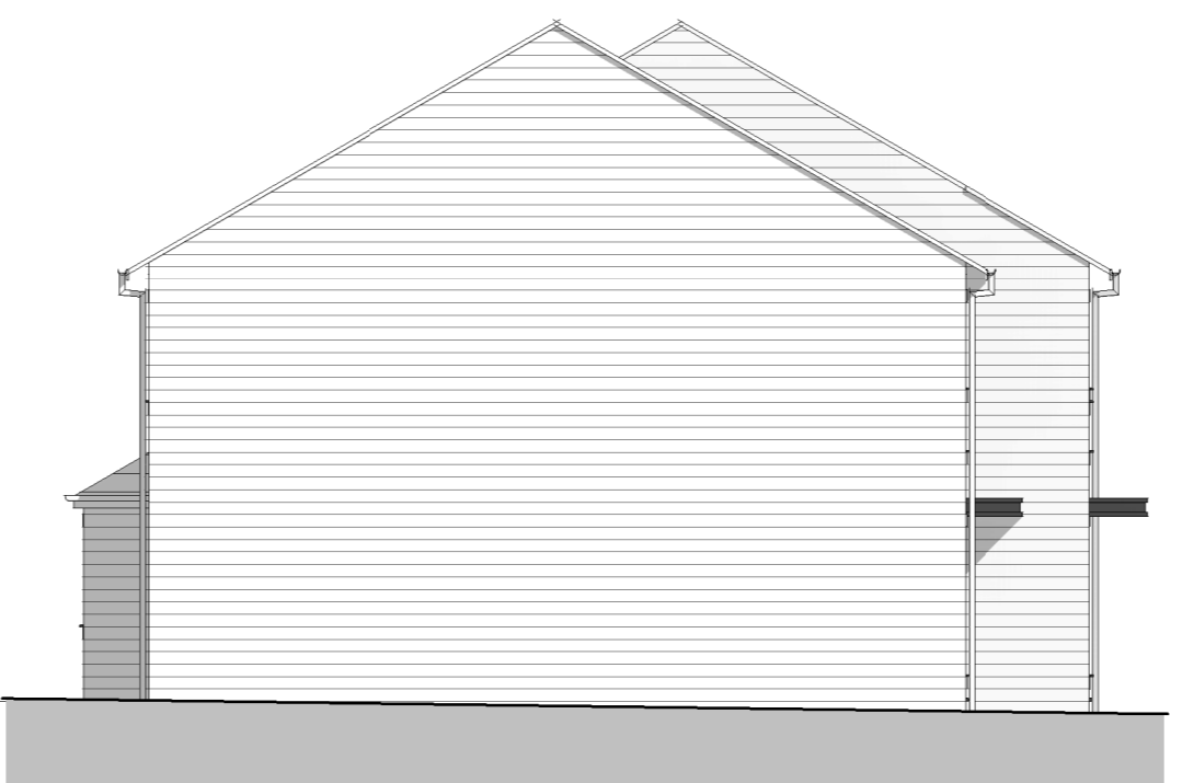
Plot 13 Side Elevation 1 : 100
