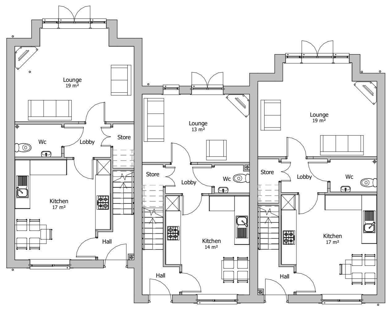
Plots 13 to 15 Ground Floor Plan 1 : 100
