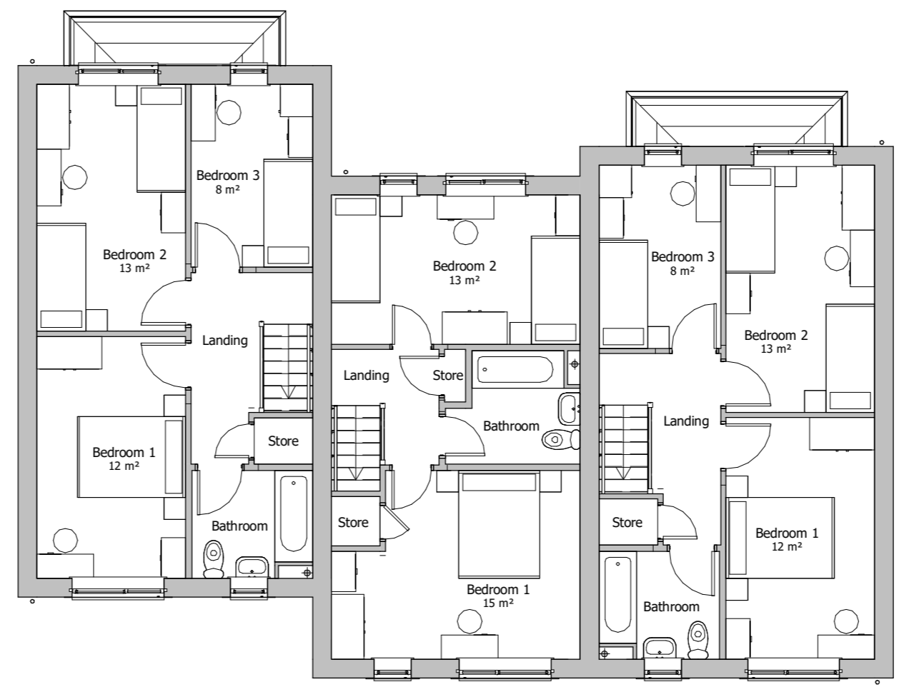
Plots 13 to 15 First Floor Plan 1 : 100
