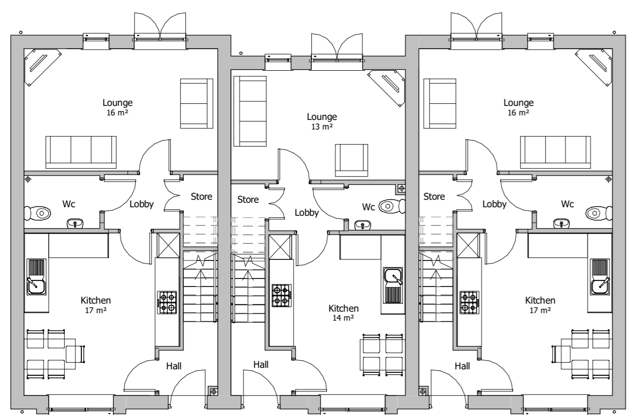
Plots 13 to 15 Ground Floor Plan 1 : 100
