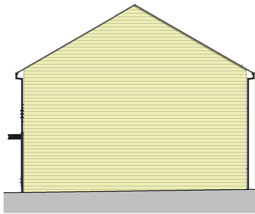
Plot 13 Side Elevation 1 : 100
