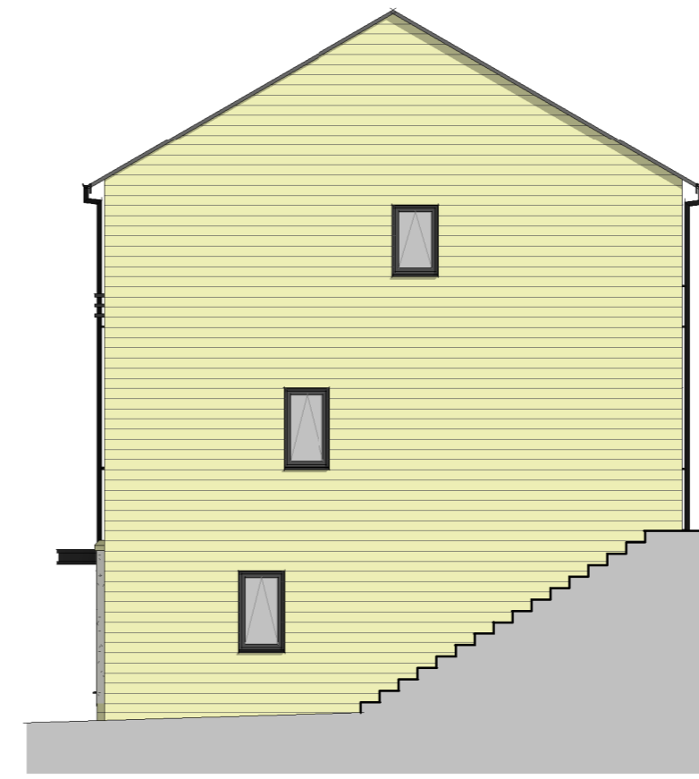
Plot 27 Side Elevation 1 : 100
