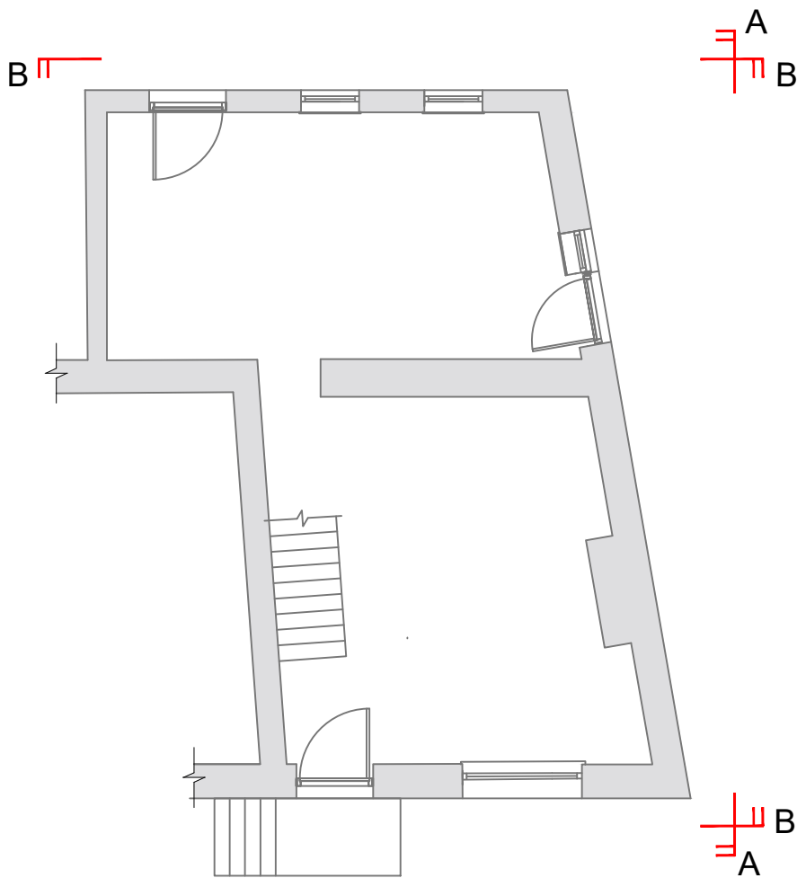
GROUND FLOOR PLAN EXISTING 1:100
