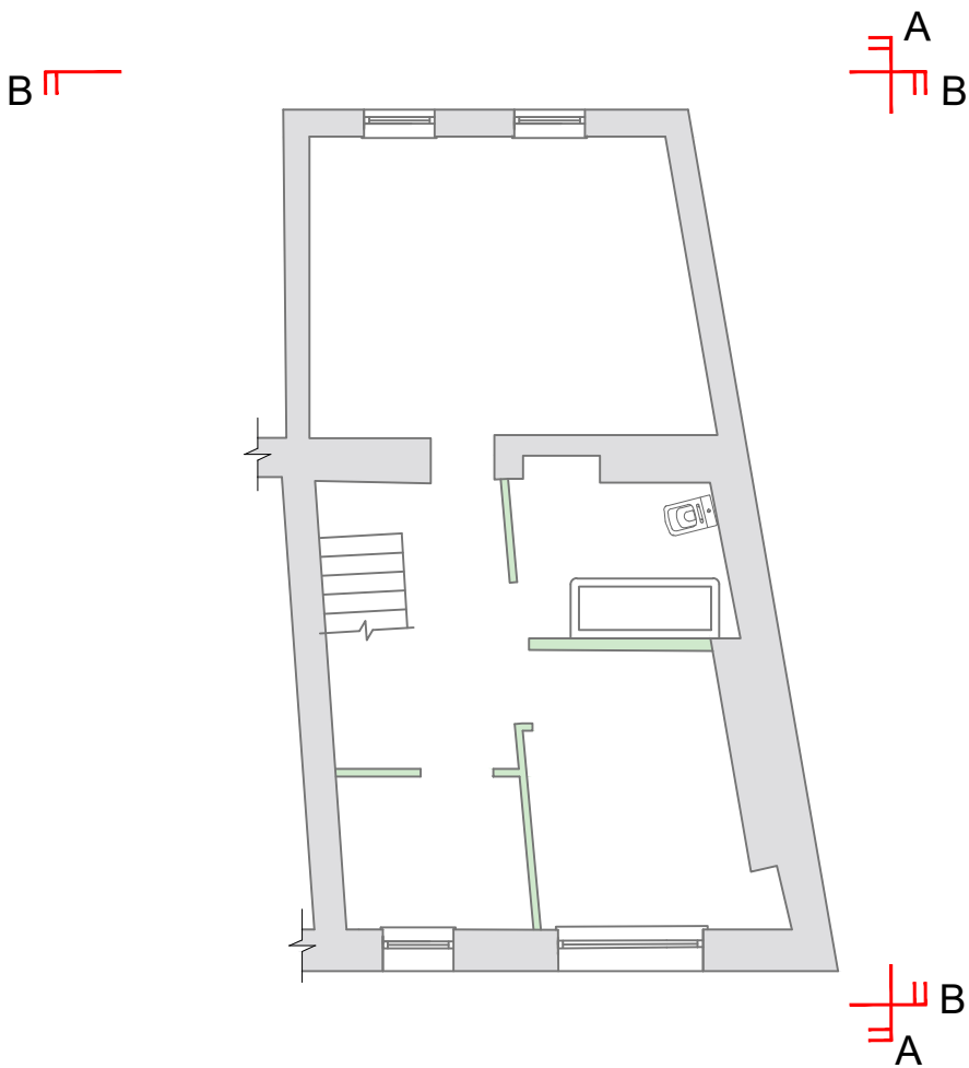
FIRST FLOOR PLAN EXISTING 1:100
