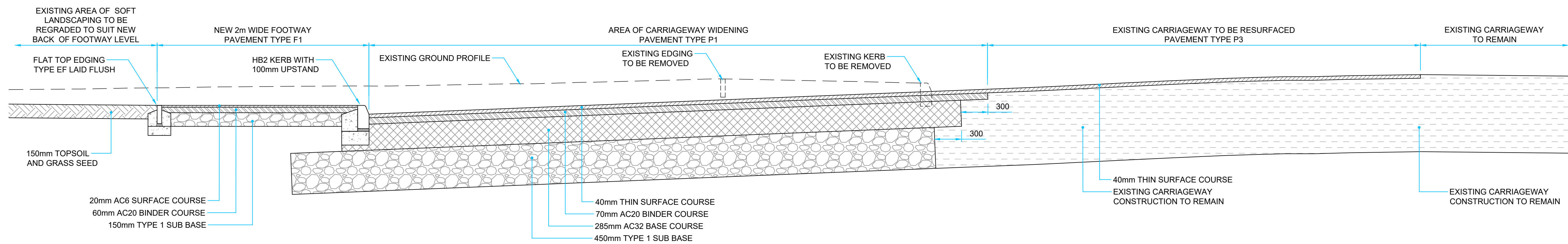
TYPICAL SECTION A - A SCALE 1:25
