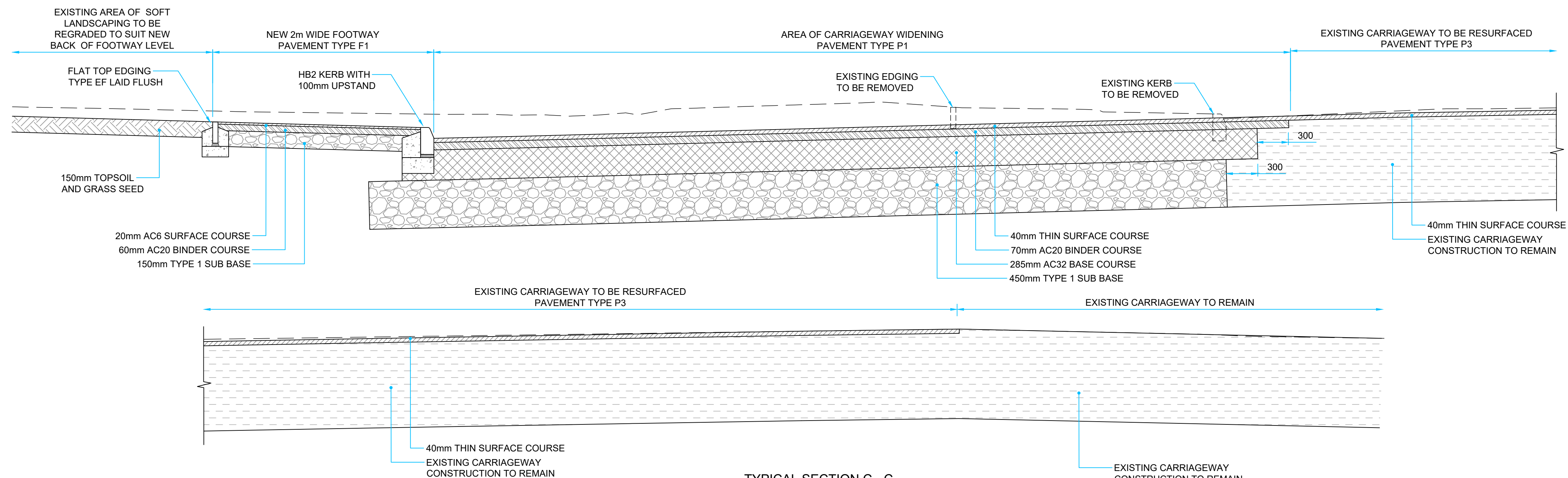
TYPICAL SECTION C - C SCALE 1:25
