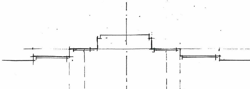
PART PLAN OF MASONRY OPENING AT FRONT DOOR
