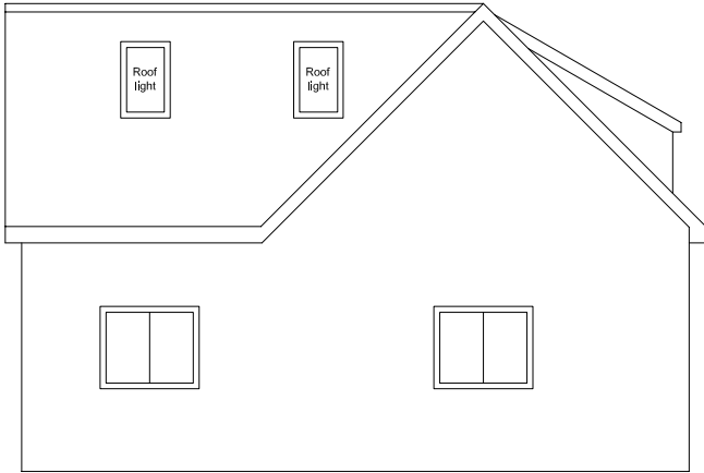
EAST ELEVATION
