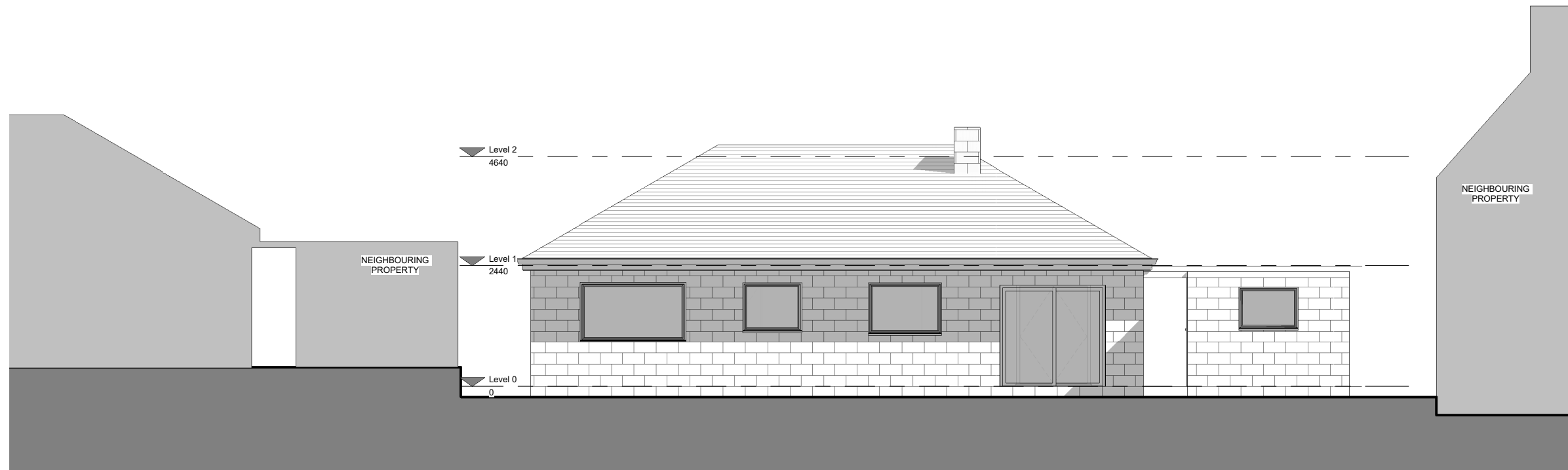
South Elevation
