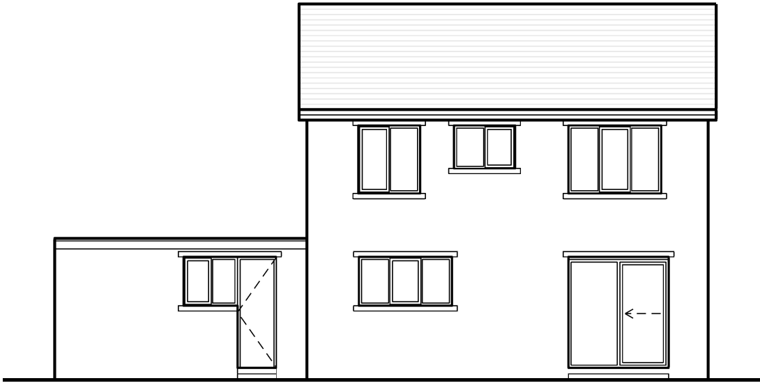
West Elevation
