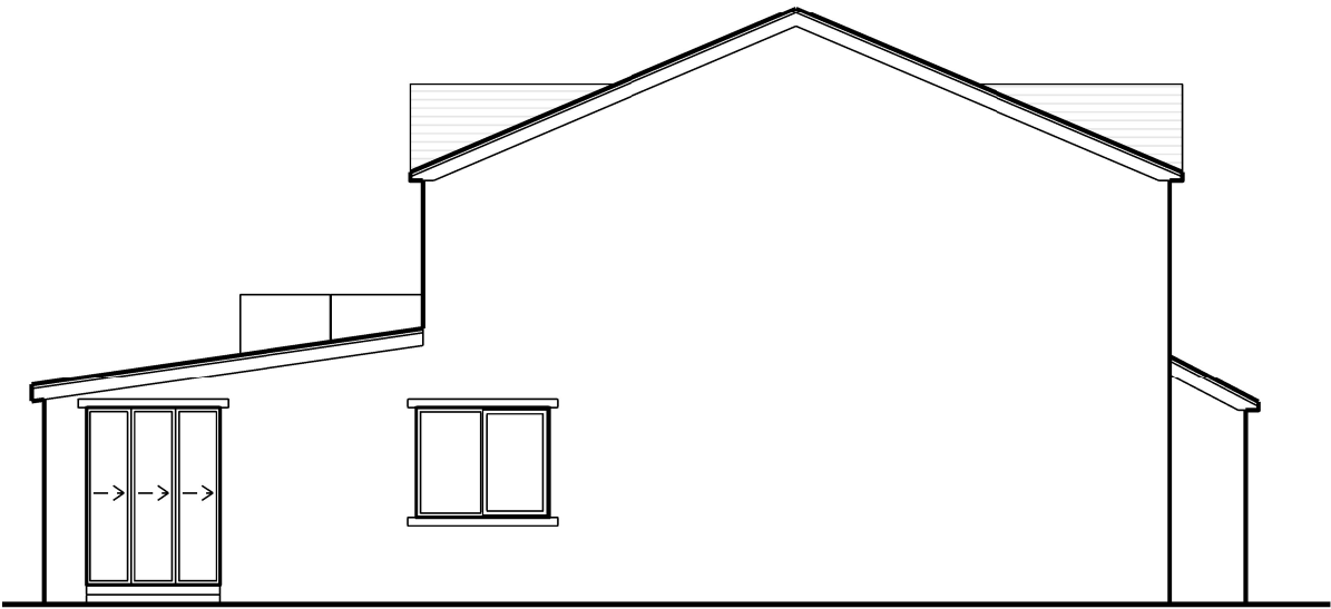
South Elevation
