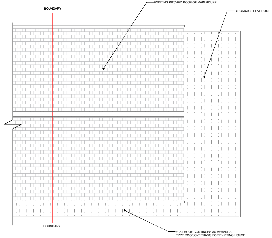
ROOF PLAN EXISTING 1:100
