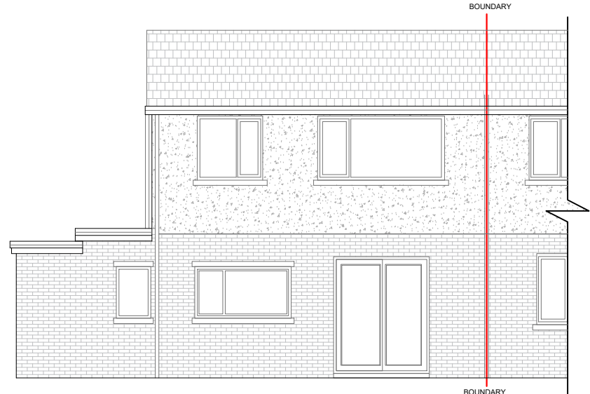
REAR ELEVATION C-C
