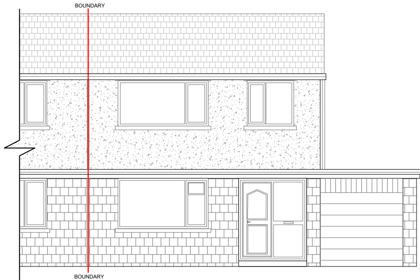
EXISTING FRONT ELEVATION A-A
