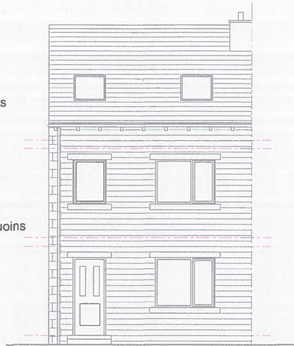
Front Elevation (plot 3)
