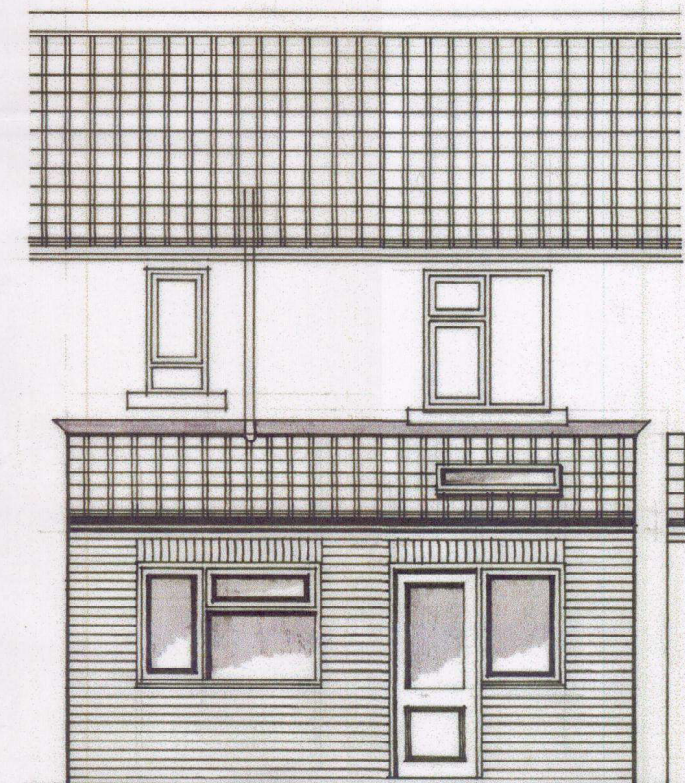
REAR ELEVATION
