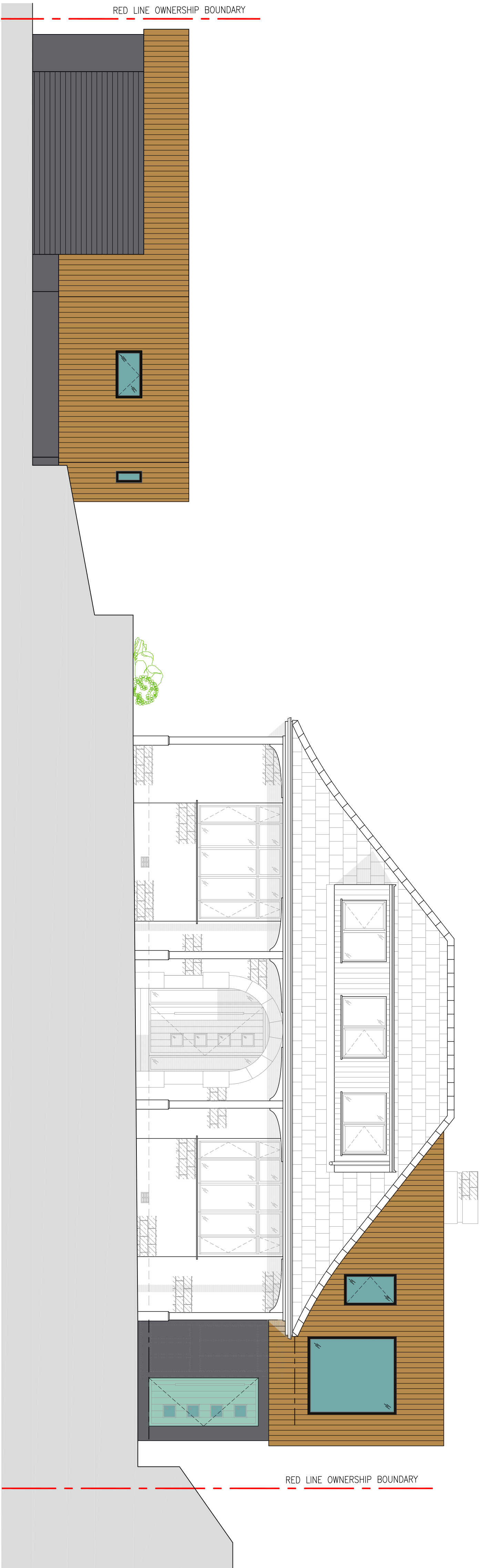
PROPOSED SOUTH WEST FACING ELEVATION SCALE 1:50
