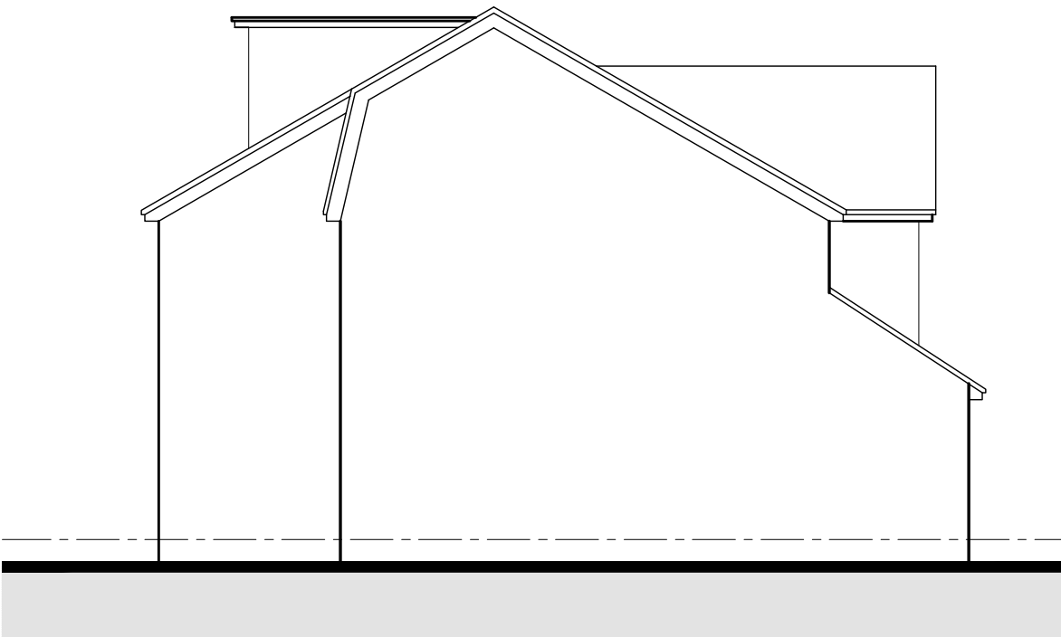
LEFT SIDE ELEVATION AS PROPOSED
