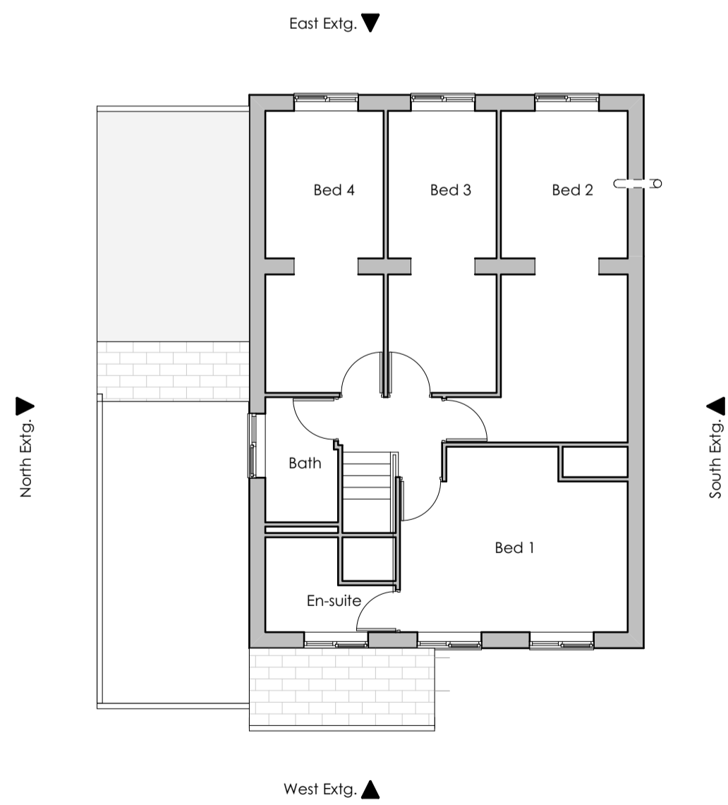
First Floor Extg.
