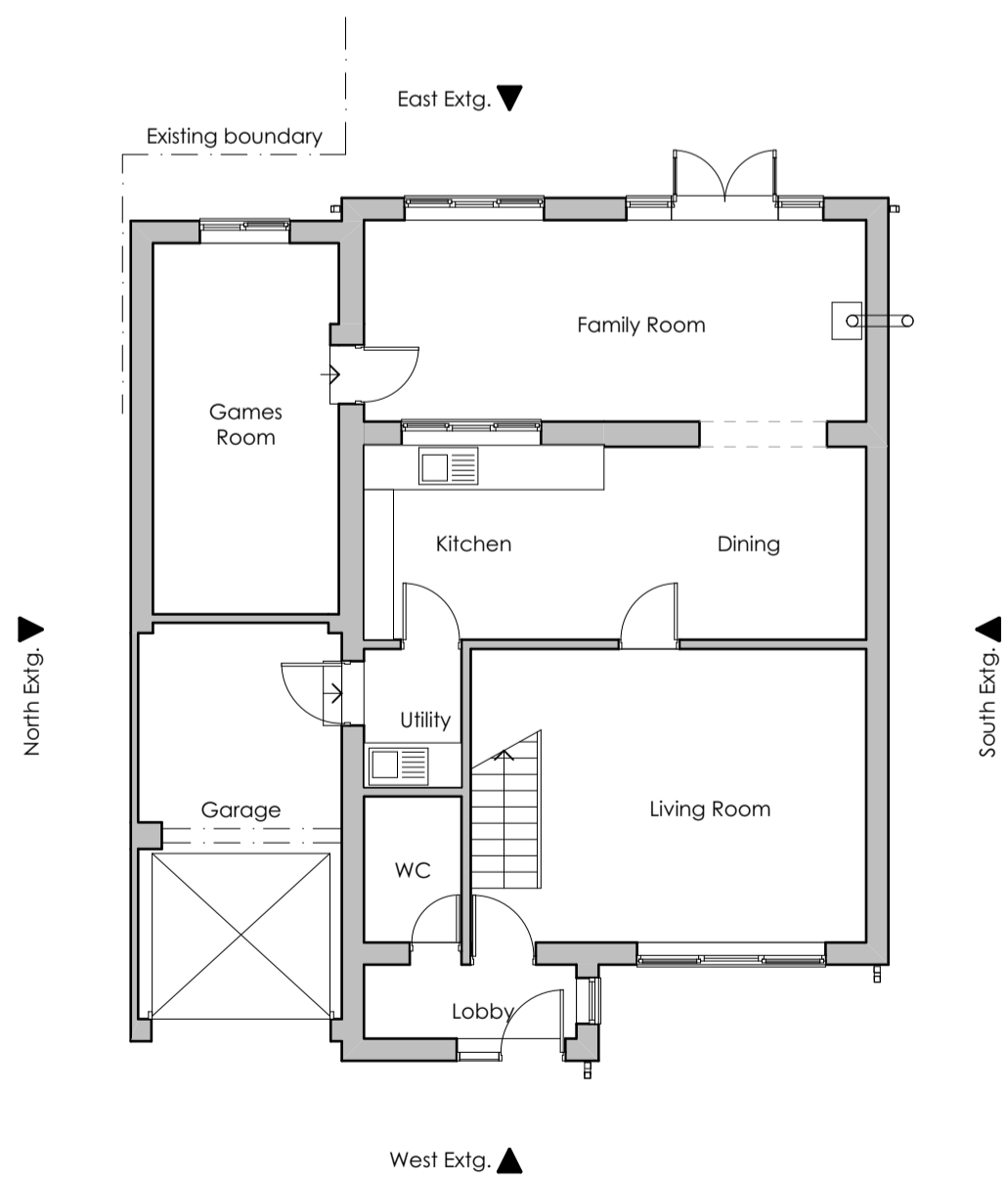
Ground Floor Extg.
