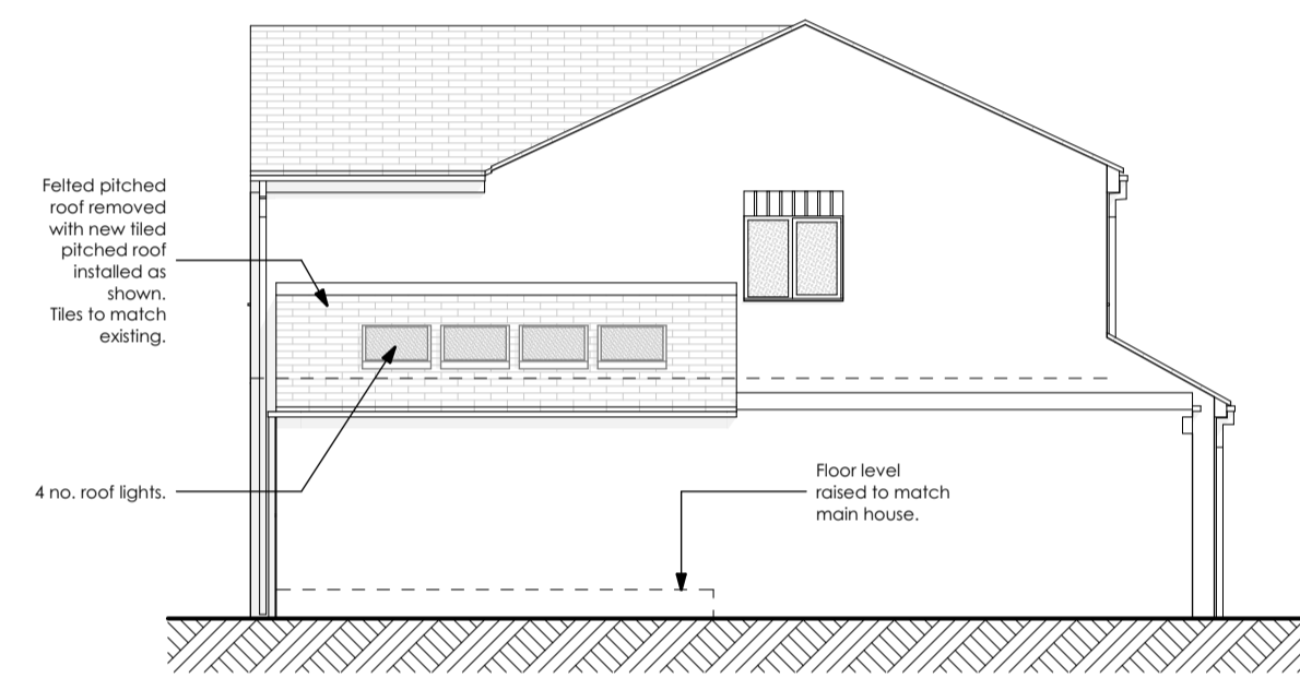
North Prop.
