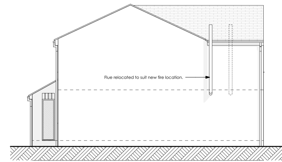
South Prop.
