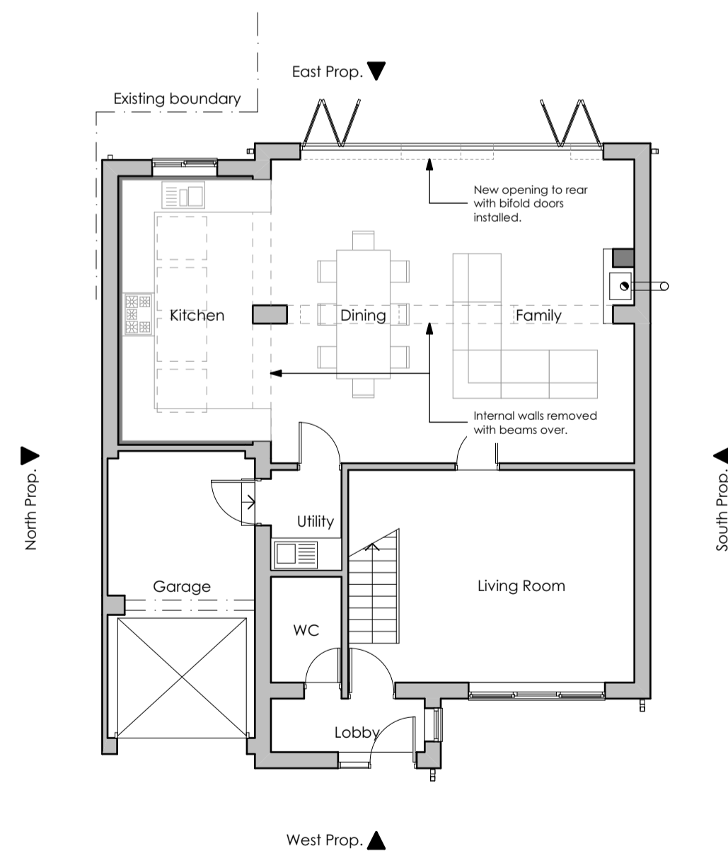
Ground Floor Prop.
