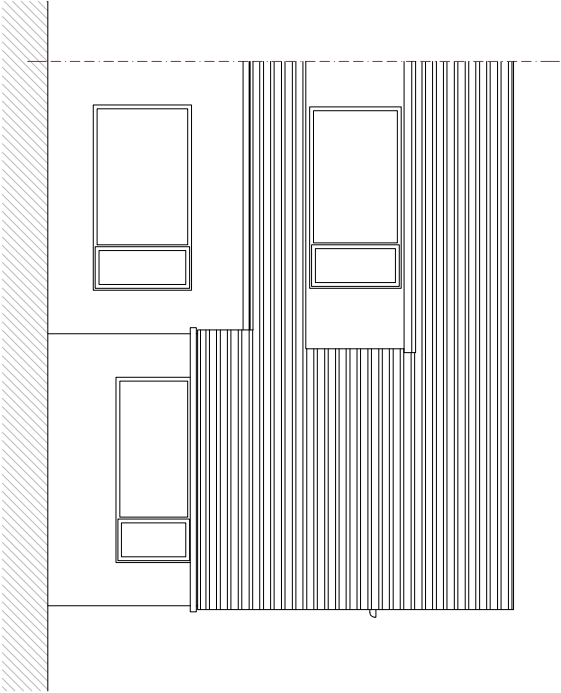
Existing Front (north) Elevation 1:100 scale
