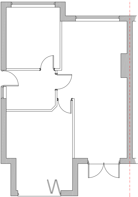
Existing Ground Floor Plan 1:100 scale
