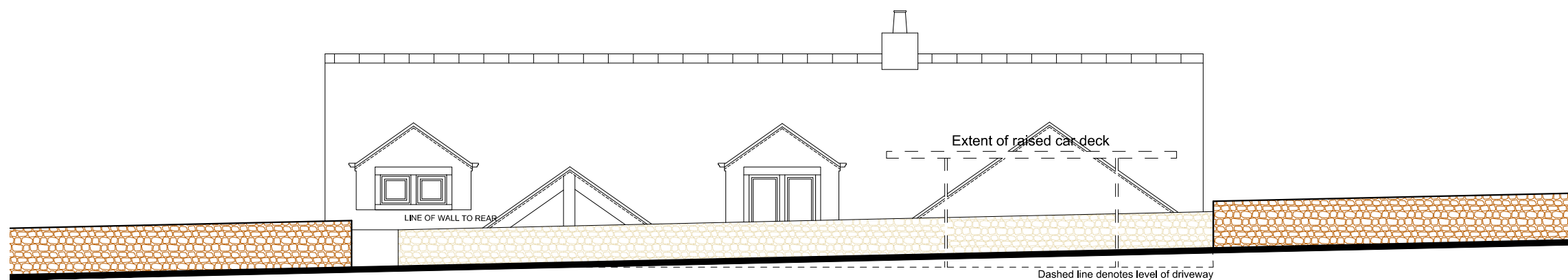
PROPOSED STREET SCENE SHOWING EXTENT OF CAR LIFT IN RAISED POSITION
