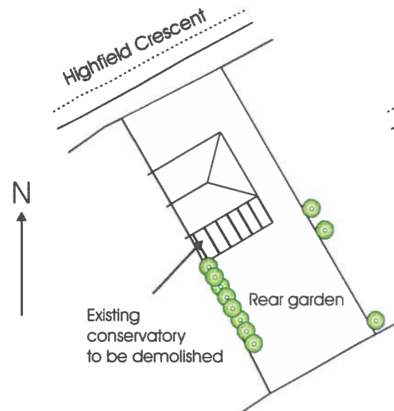
Block Plan (existing) Scale 1 : 500
