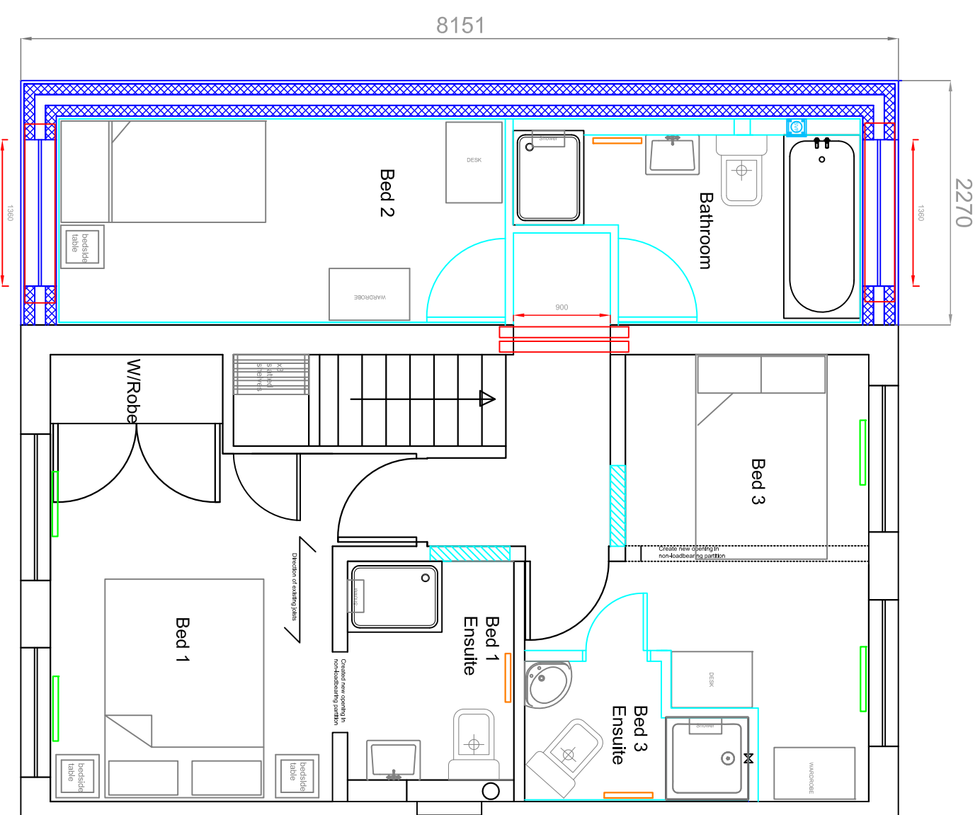
14 Kirk Close, Dewsbury, WF12 8RJ Proposed 1st Floor Layout
