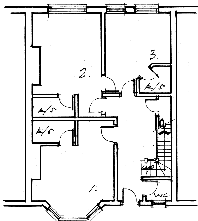
PROPOSED GROUND.
