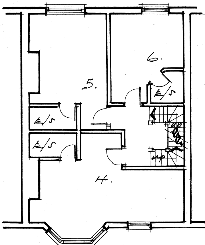
FIRST.
