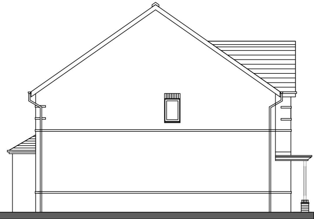
SIDE ELEVATION
