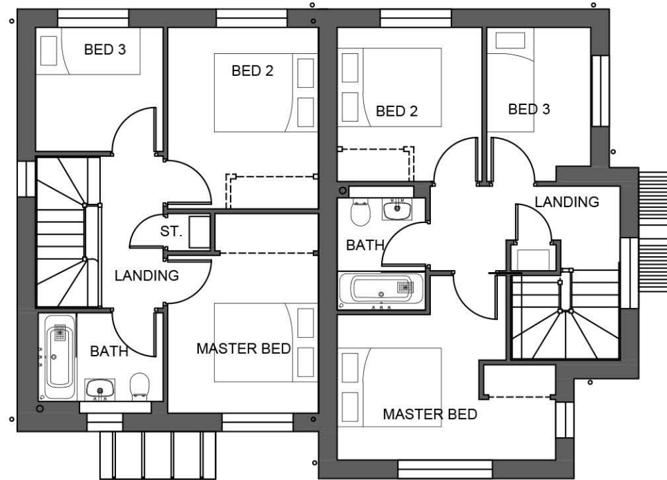
FIRST FLOOR PLAN Bampton
