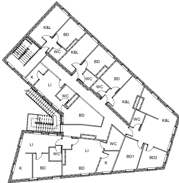
1 First Floor 1 : 100
