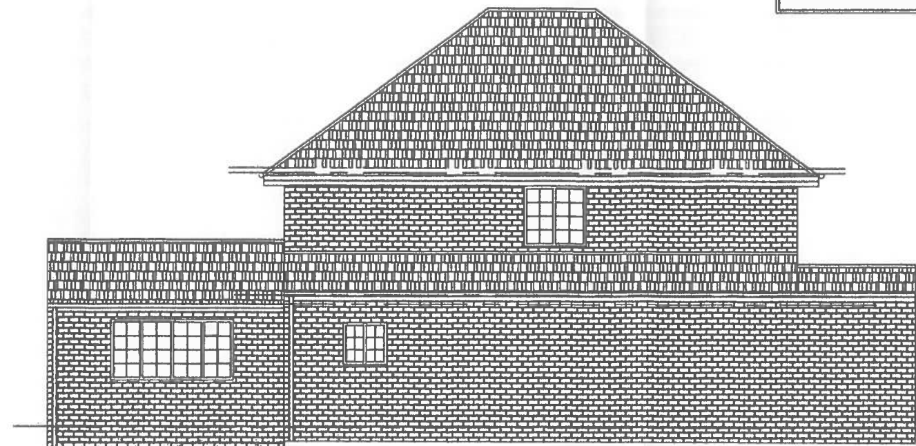
Existing Left Side Elevation 1:100
