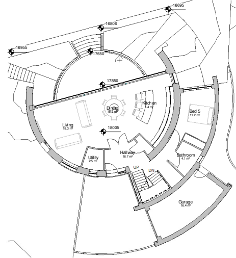
00-Ground Floor Scale 1 : 100
