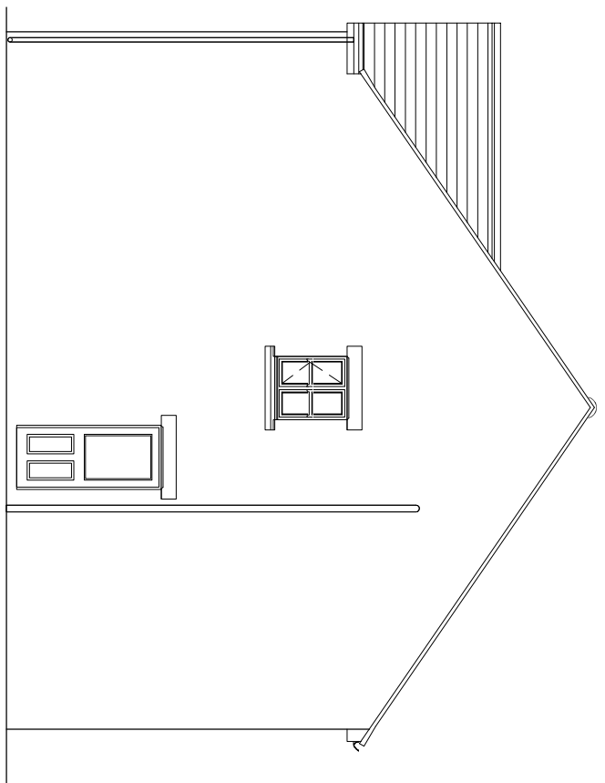
Side Elevation
