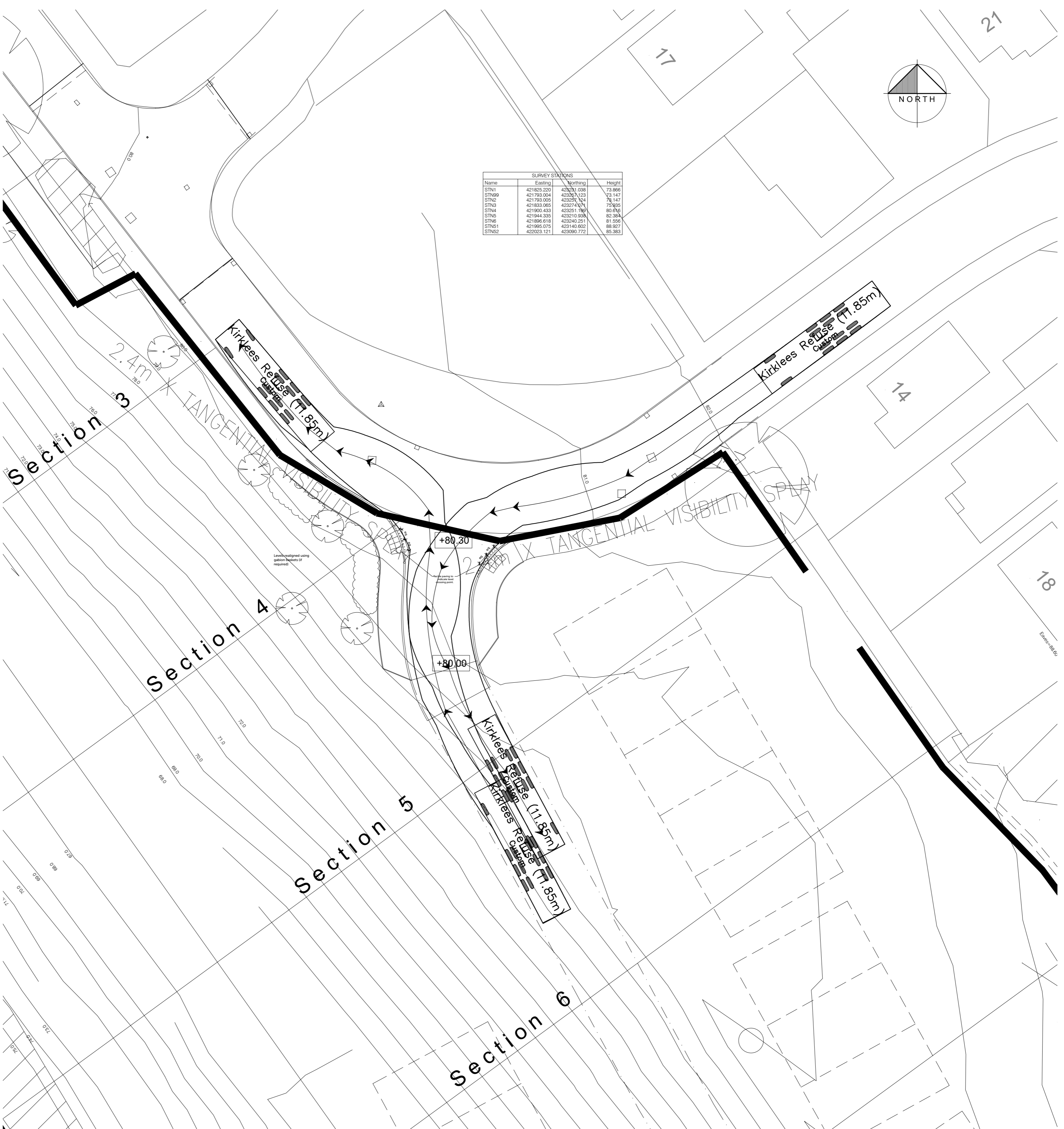
Site Plan 1:200 @ A1
